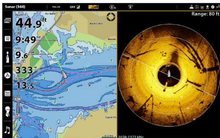
360/Chart View [SOLIX]
