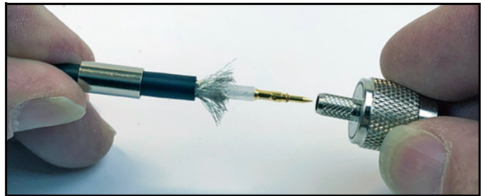
Figure 53: Pushing On the Connector
