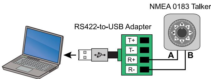
Figure 63: Connecting a NMEA 0183 Talker to a Laptop
