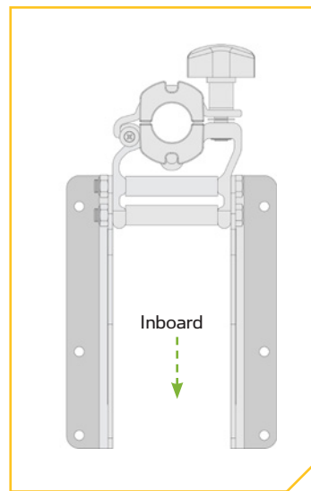
PowerDrive Pontoon Hand Control Bracket
