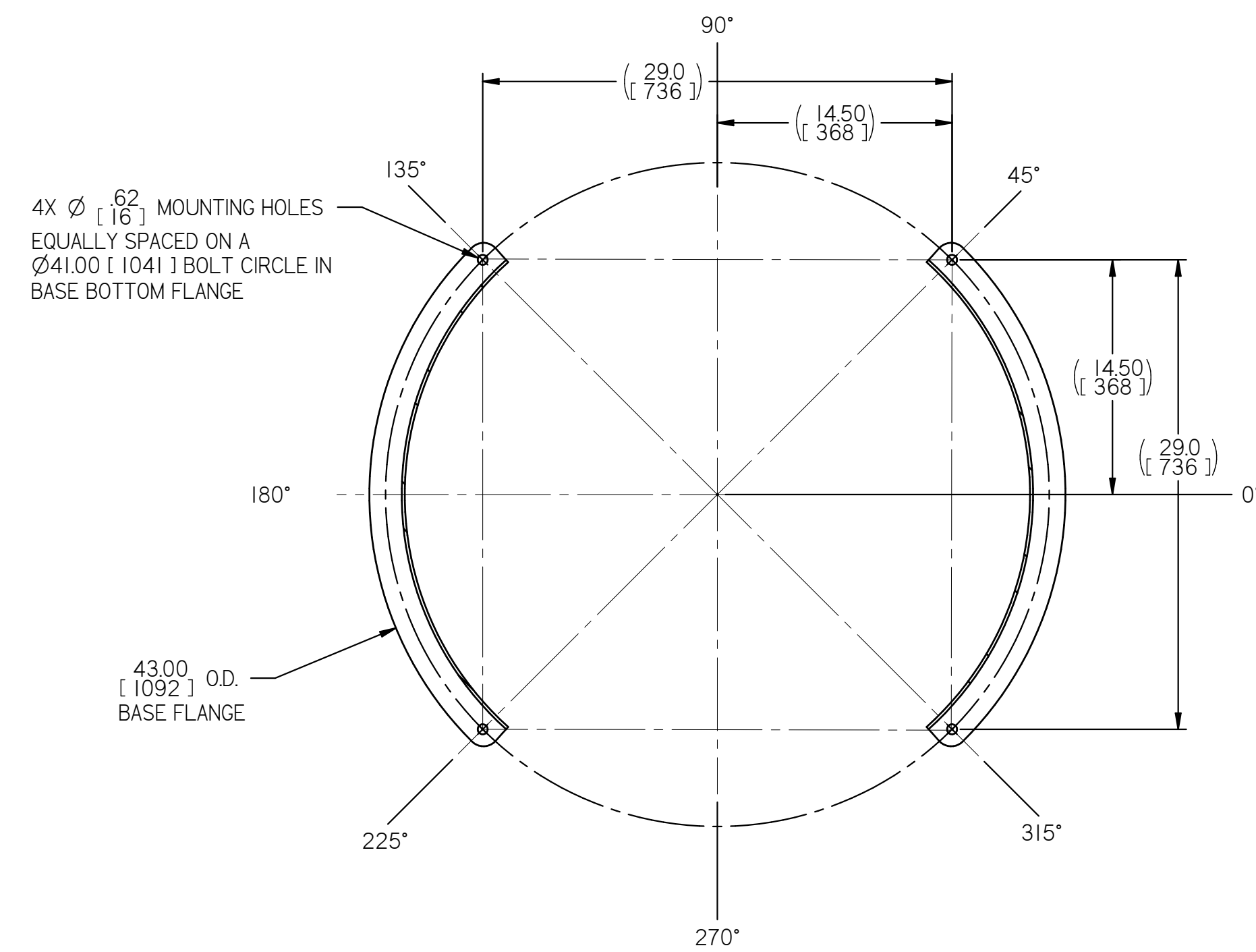
UNIT MOUNTING DETAILS 1:8
