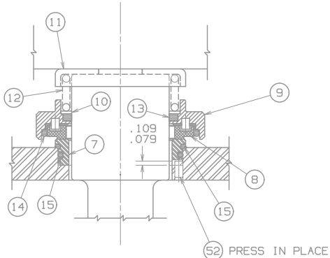
VIEW SHOW NG SEAL FULL SCALE
