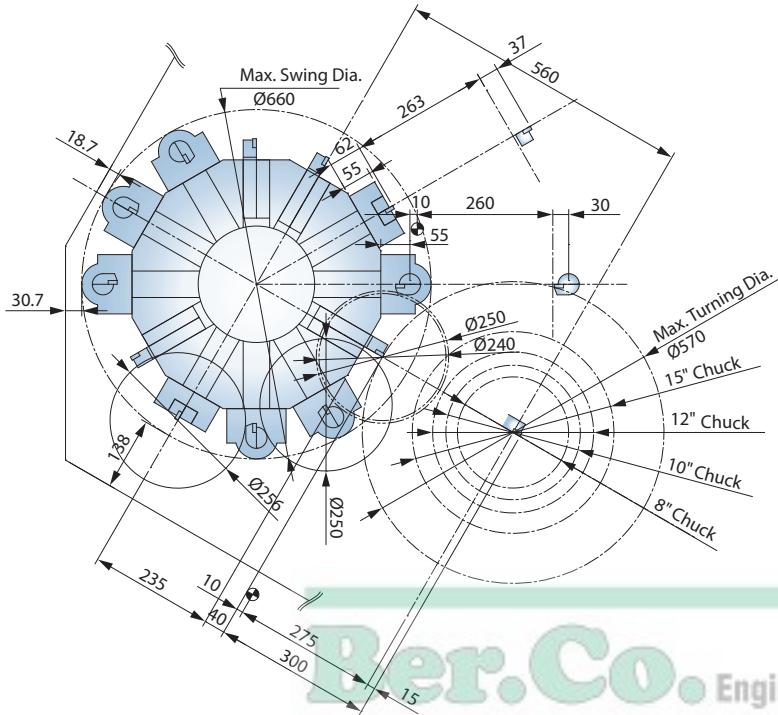
[ 12-Station Turret ]
