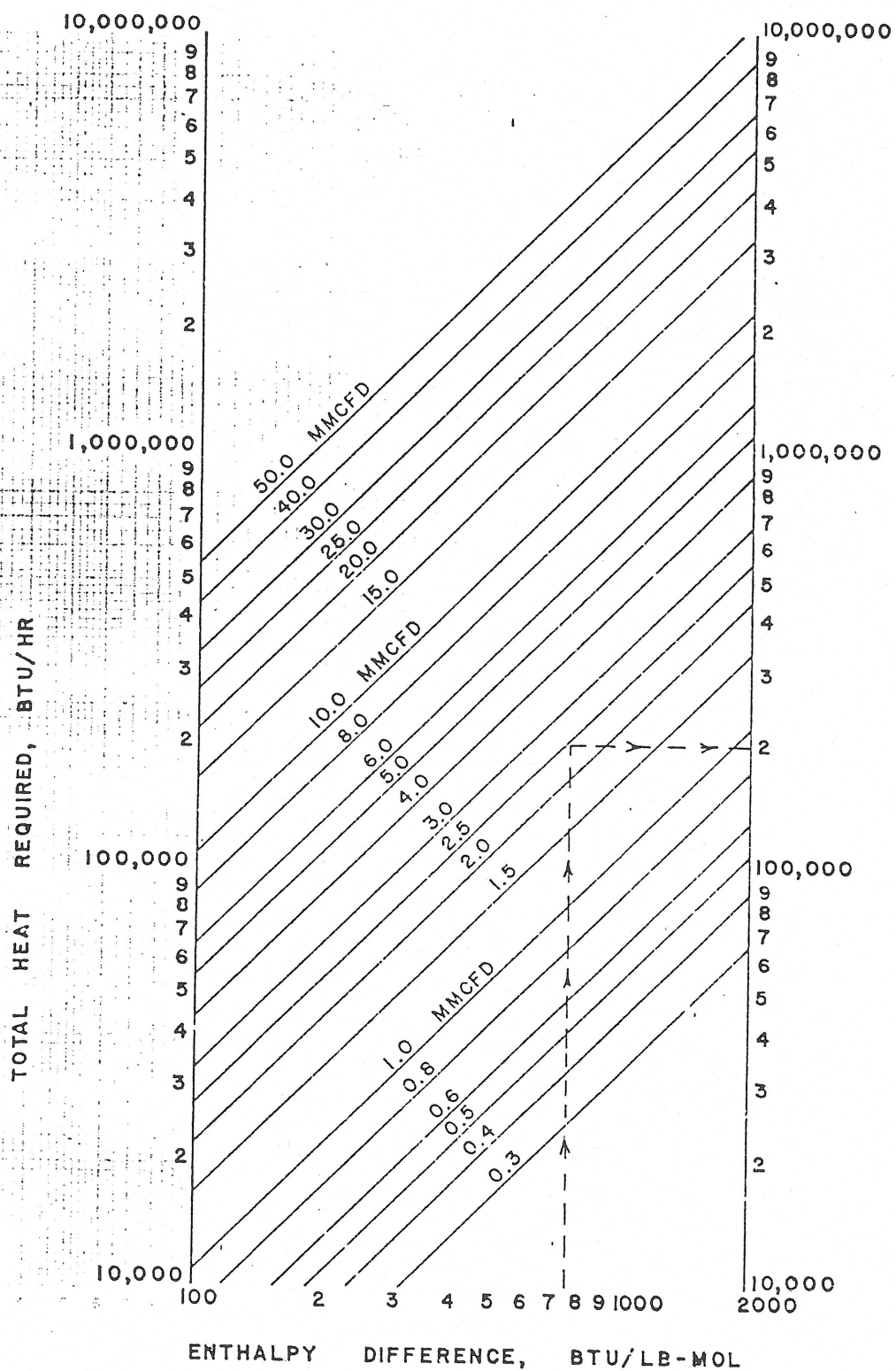
FIGURE 2 HEAT REQUIRED FOR NATURAL GAS
