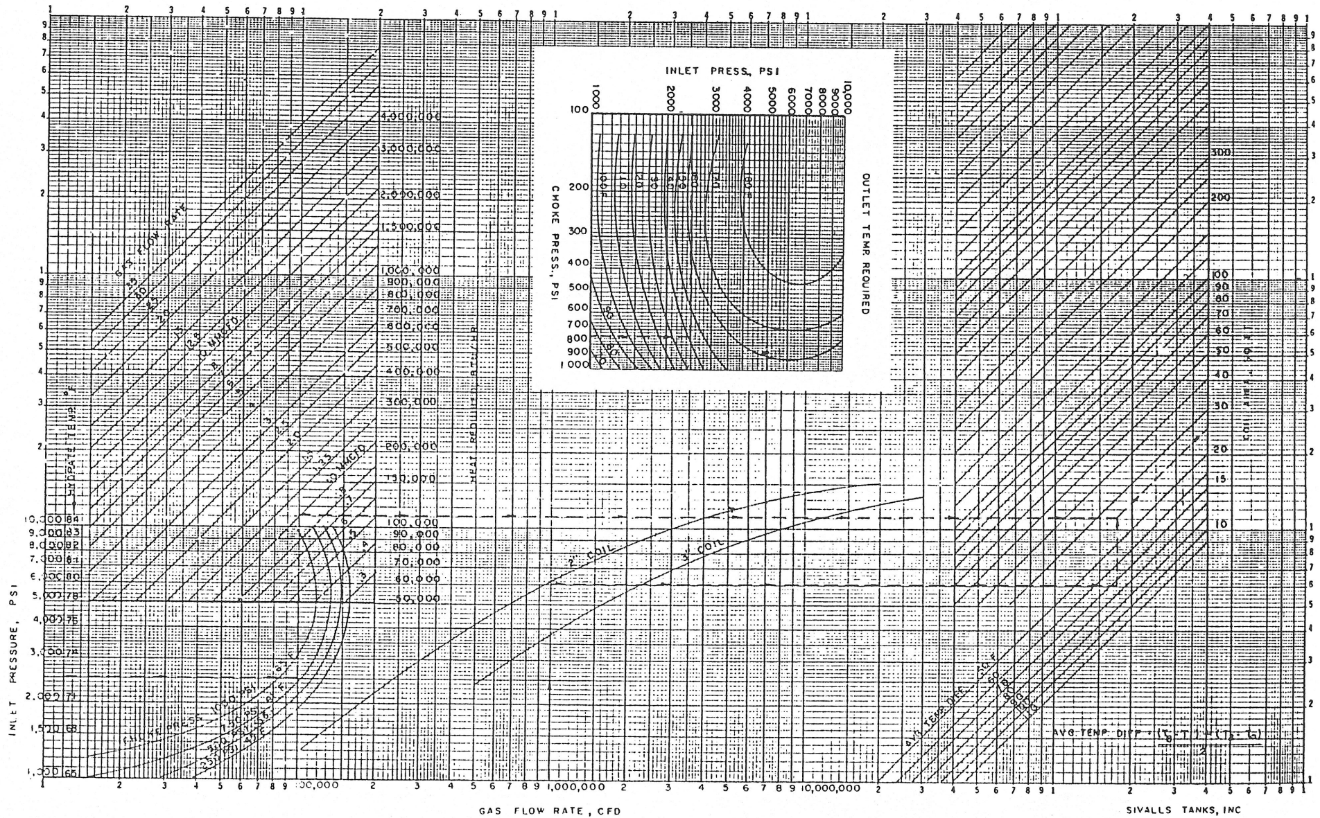
FIGURE 6 SIZING CHART FOR NATURAL GAS INDIRECT HEATER SP. GR. = 0.7
