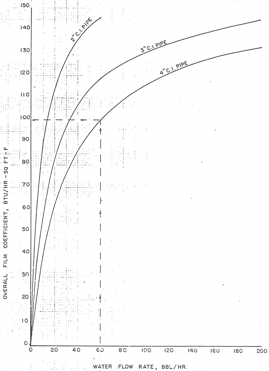
FIGURE 3A OVERALL FILM COEFFICIENT FOR WATER IN INDIRECT HEATERS
