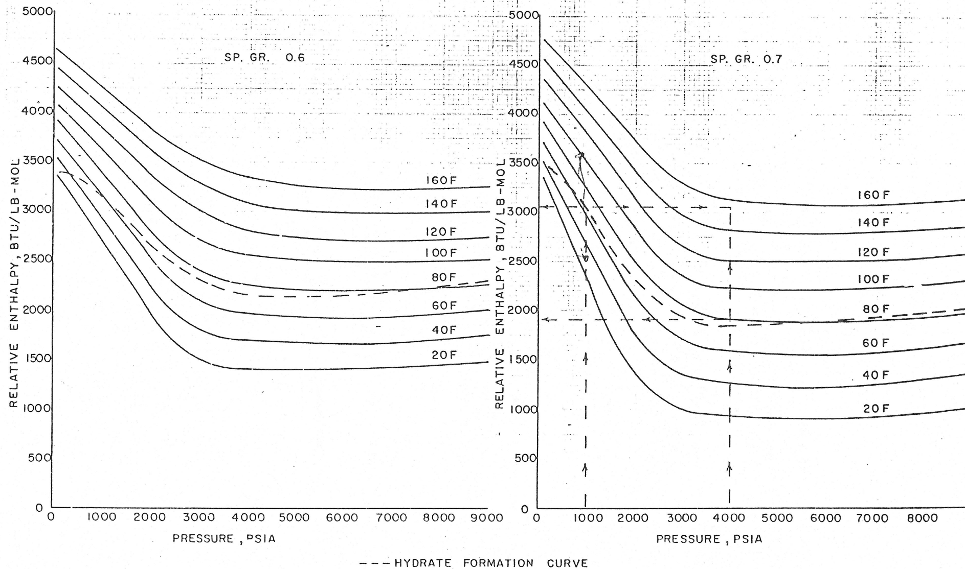
FIGURE 1 PRESSURE - TEMPERATURE - ENTHALPY CURVES FOR NATURAL GAS
