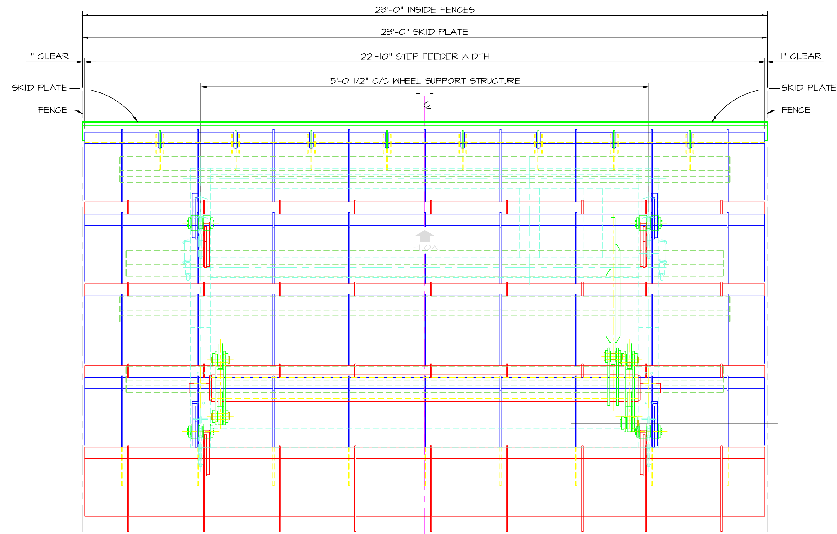
PLAN 1/2"=1'-0"
