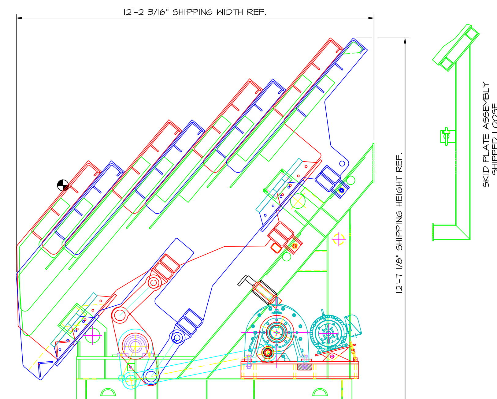
SHIPPING DIMENSIONS 1/2"=1'-0"
