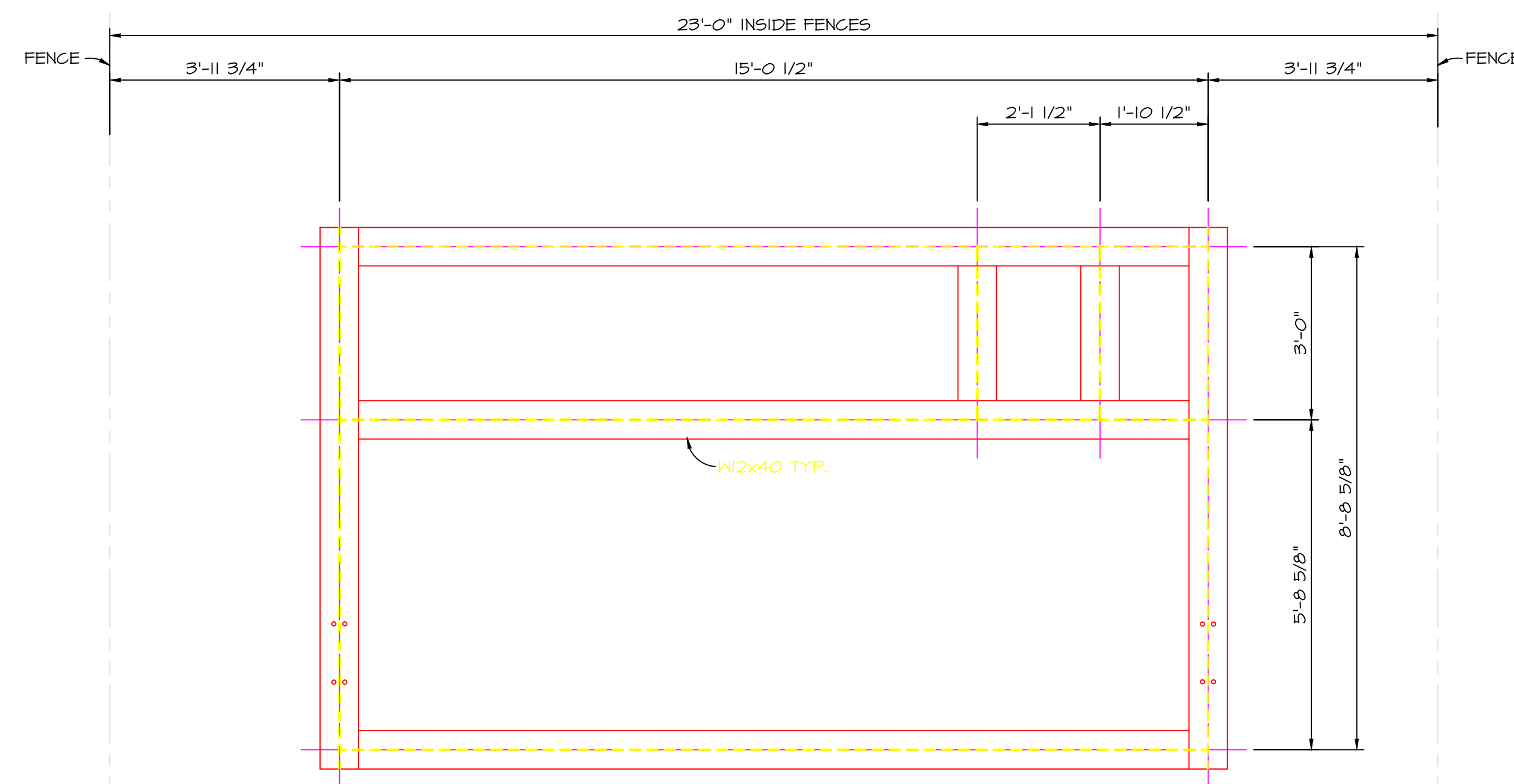
FRAME PLAN 1/2"=1'-0"
