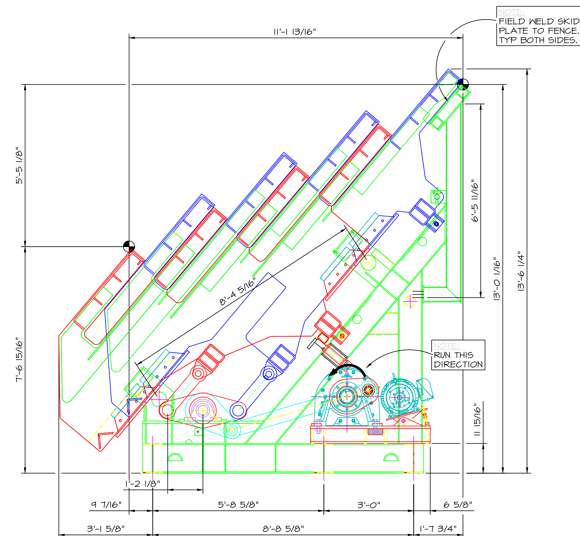
ELEVATION 1/2"=1'-0"
