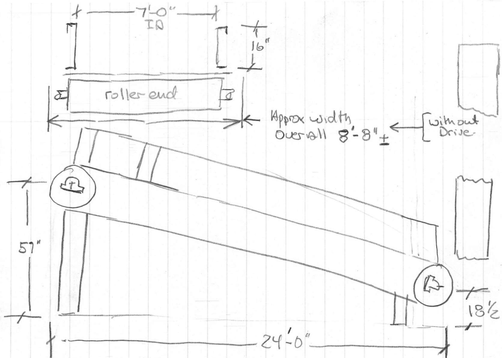
SIDE VIEW IMPCO Conveyor
