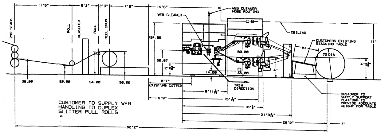
ELEVATION VIEW
