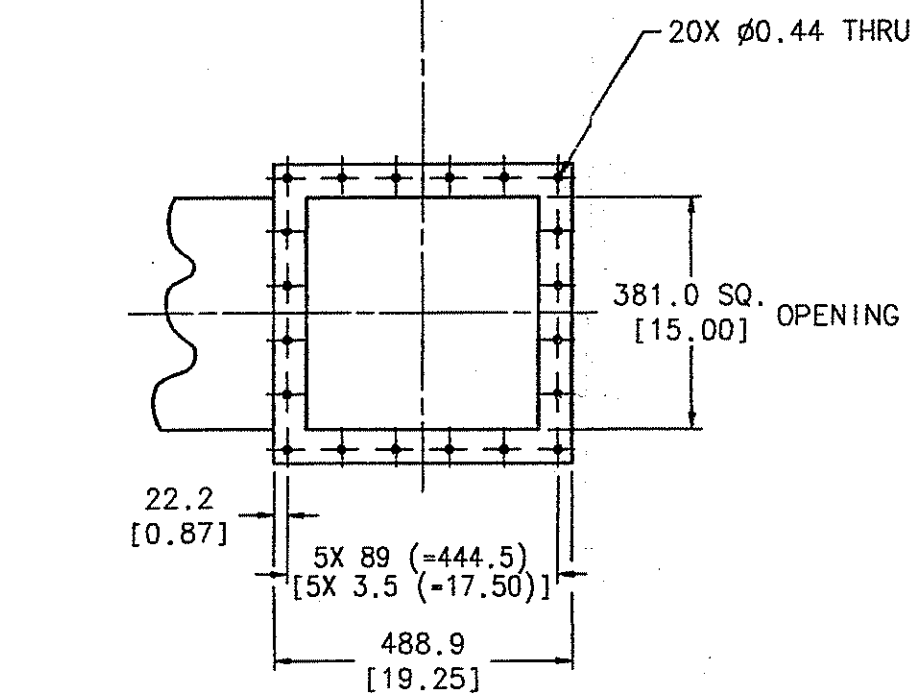
CONVEYOR DISCHARGE FLANGE
