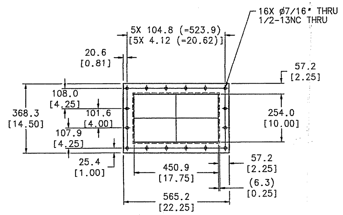
DRAIN DETAIL
