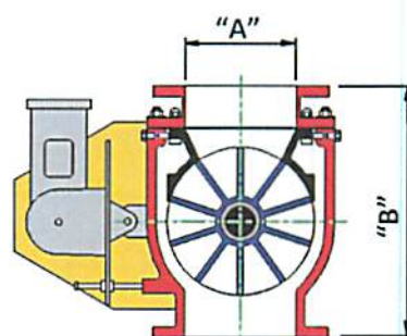
XT Rotary Valve
