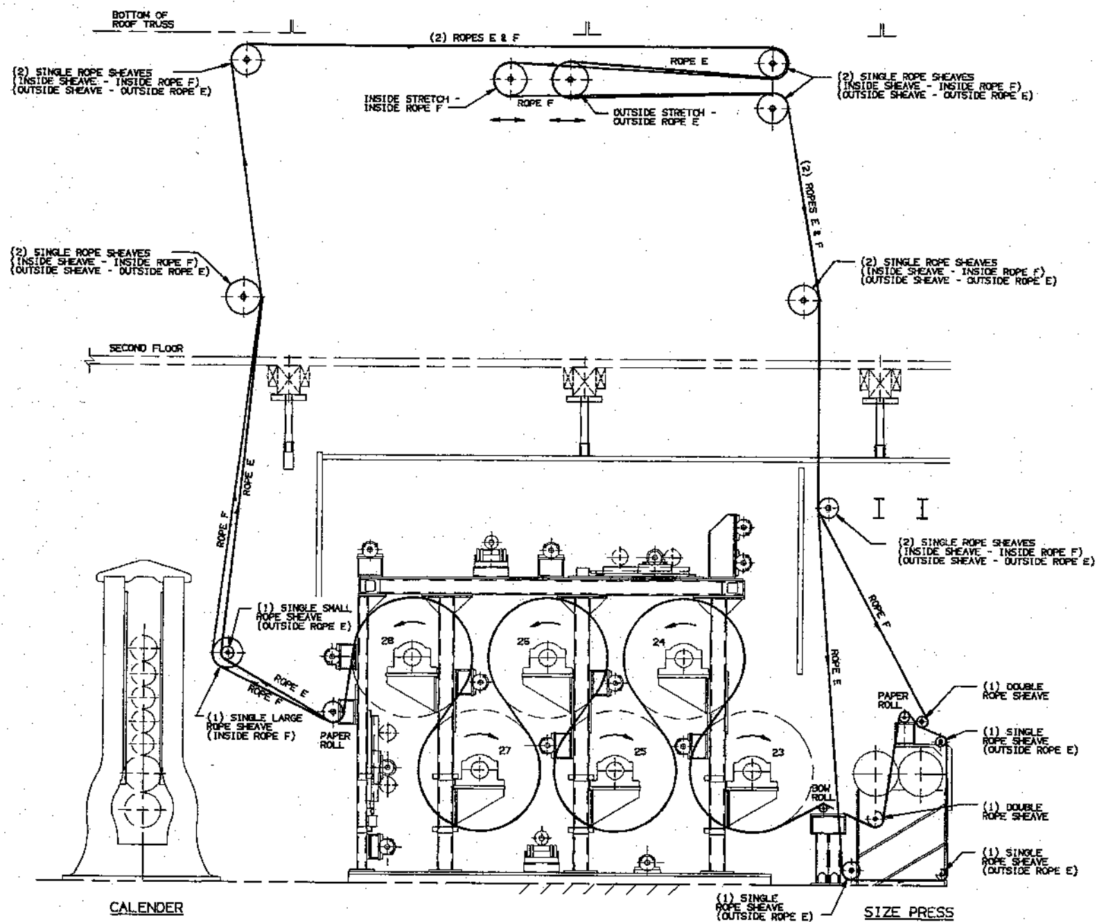
ROPE SYSTEM - THIRD DRYER SECTION TENDING SIDE ELEVATION
