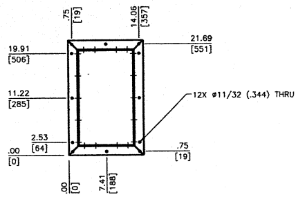
PORT B FLANGE CONNECTION
