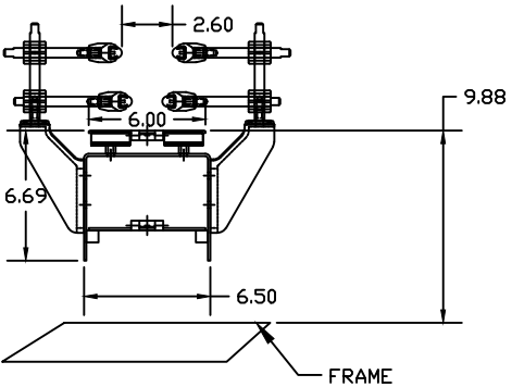
CONVEYOR SECTION THROUGH MACHINE CHAIN: LF820K6 (3X SCALE)
