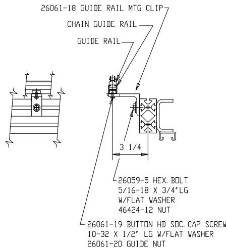
VIEW S CHAIN GUIDE MOUNTING SEE CONVEYOR DRIVE SIDE ELEVATION SCALE = 1/4
