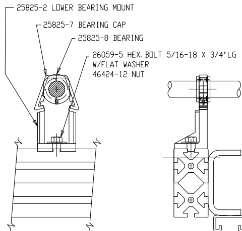
VIEW T LOWER CONVEYOR ROLL BEARINGS FROM CONVEYOR DRIVE SIDE ELEVATION SCALE = 1/2
