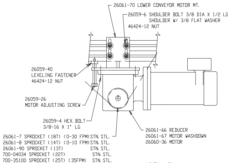
VIEW P LOWER CONVEYOR MOTOR MOUNT FROM CONVEYOR DRIVE SIDE ELEVATION SCALE = 1/4
