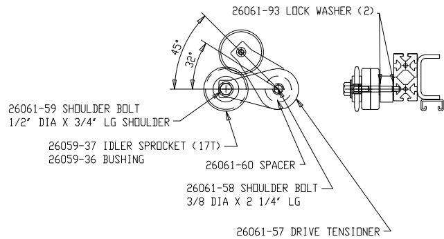
VIEW V DRIVE TENSIONER FROM CONVEYOR DRIVE SIDE ELEVATION SCALE = 1/4
