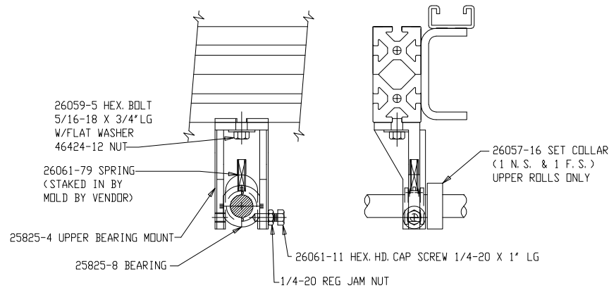
VIEW U UPPER CONVEYOR ROLL BEARINGS FROM CONVEYOR DRIVE SIDE ELEVATION SCALE = 1/2
