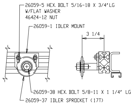
VIEW Q TYP DRIVE IDLER FROM CONVEYOR DRIVE SIDE ELEVATION SCALE = 1/4
