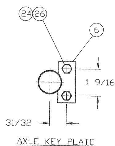
AXLE KEY PLATE
