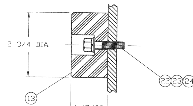
BUMPER SECTION
