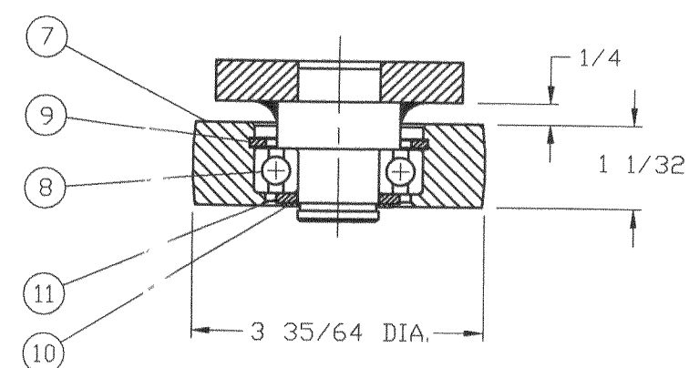
GUIDE ROLLER SECTION
