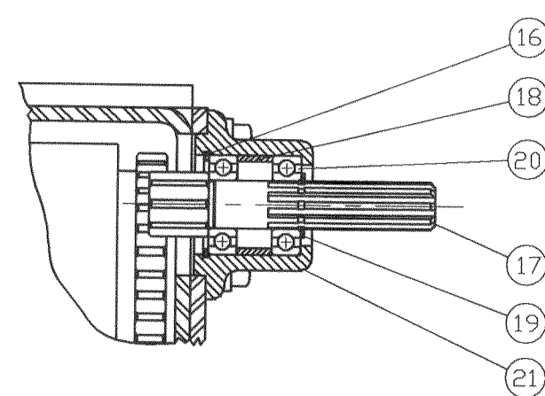
SECTION C-C
