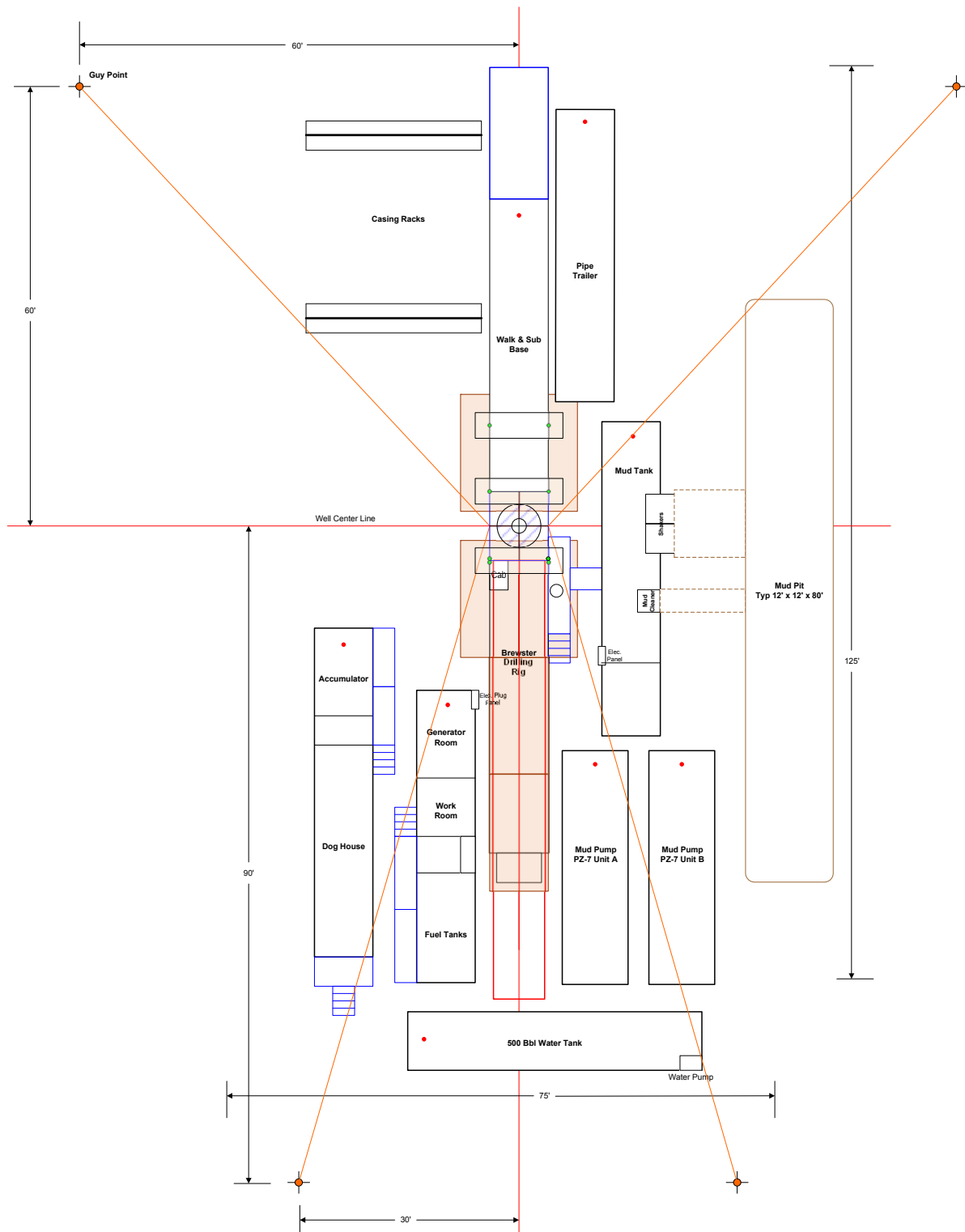
RIG #1 TYPICAL RIG LAYOUT DRAWING Red Dot = Trailer King Pin 02/18/2013 SFC
