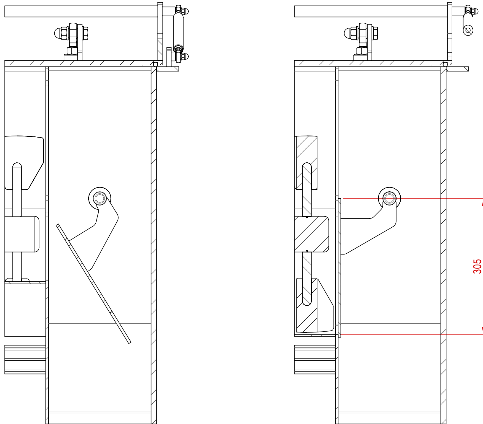
SECTION B-B SCALE 1:5
