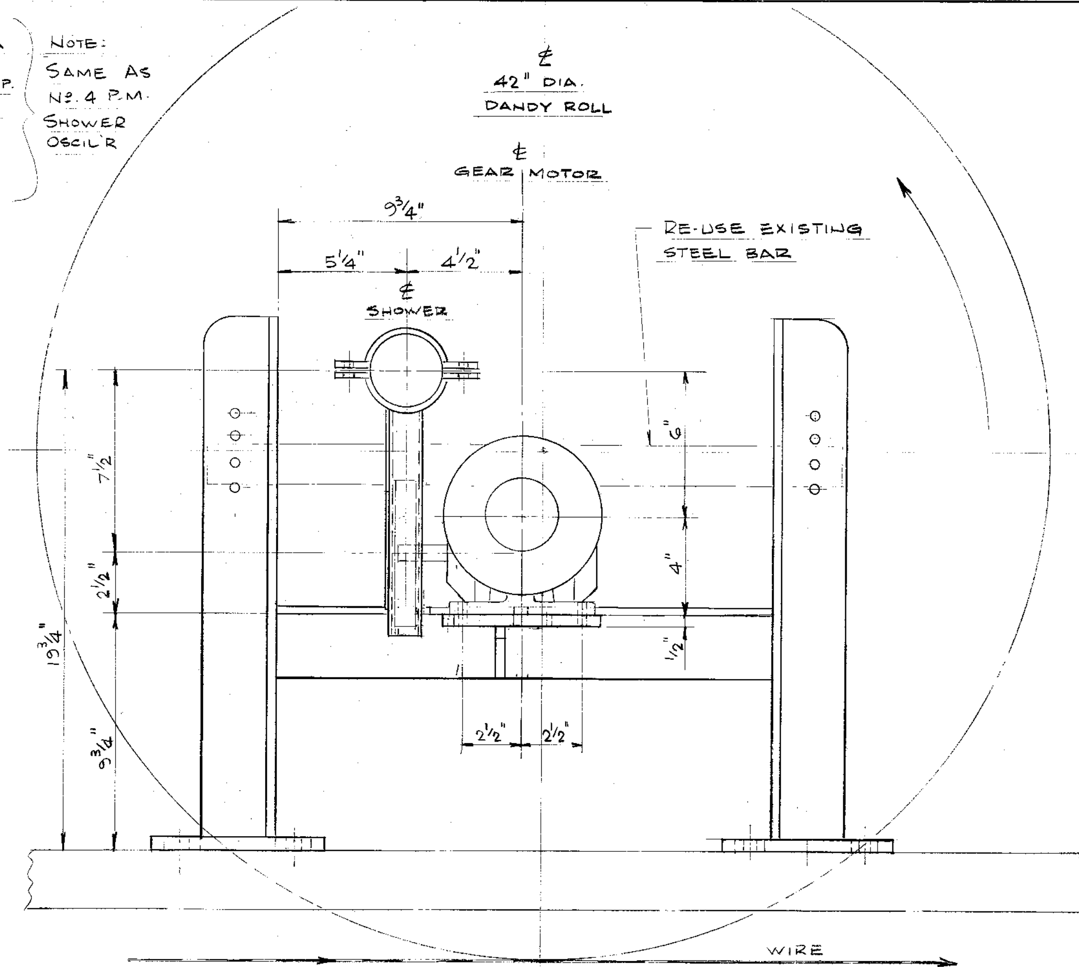
TENDING SIDE - ELEVATION VIEW
