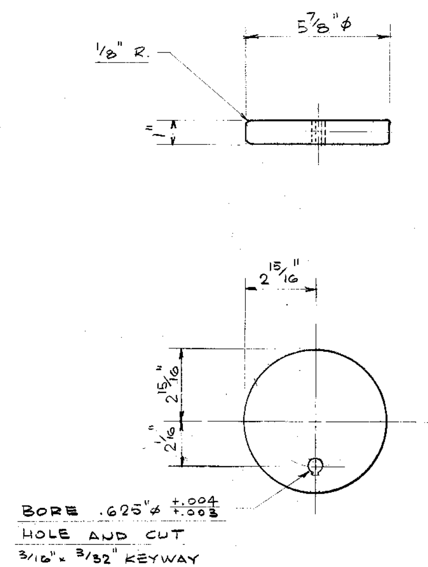
CAM WHEEL ONE REQ'D, MAT'L: BRONZE
