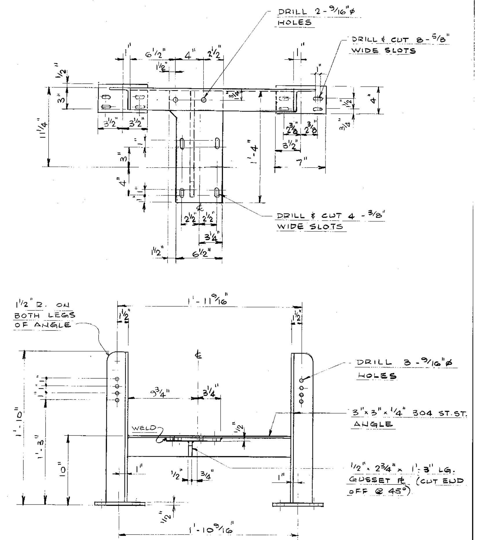
SHOWER OSCILLATOR STAND ONE REQ'D, MAT'L: 304 ST. ST.
