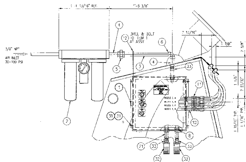
VIEW "A-A"
