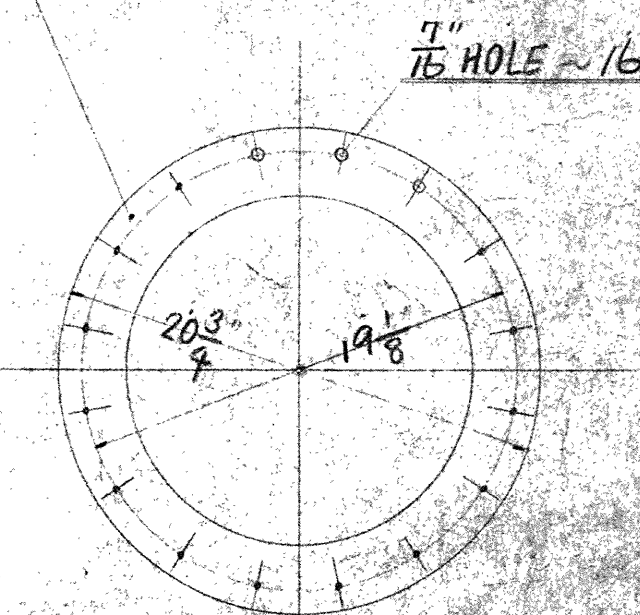
A - A VIEW
