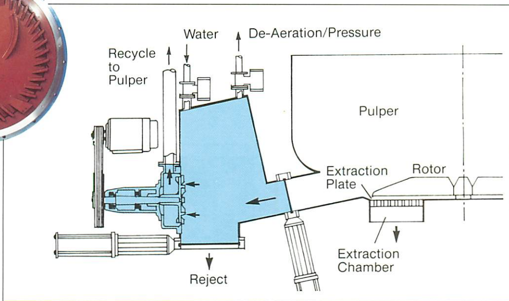
Trash extracted with a Scavenger from an 18' pulper.
