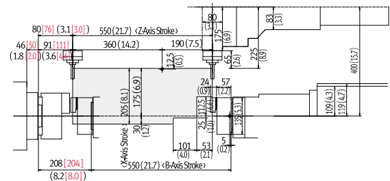
Single ID Tool Holder
