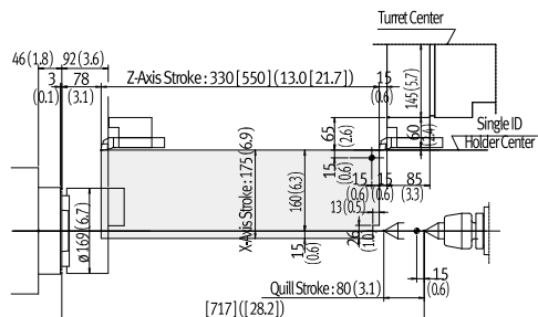
Face Tool Holder
