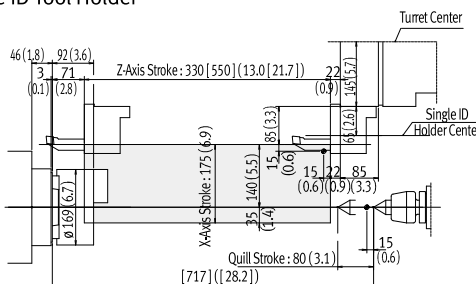
Double ID Tool Holder
