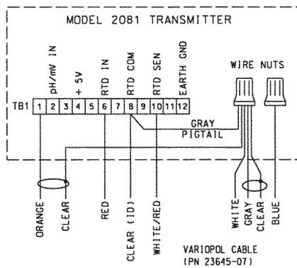
FIGURE 4-5. Wiring Details for Models 396PVP or 396P-02-54 with Mating Variopol Cable (PN 23645-07) for use with Model 2081
