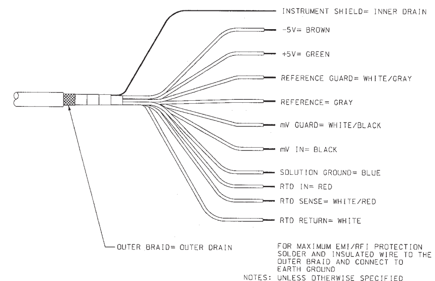
Model 396P Option 01 (with preamplifier) cable
