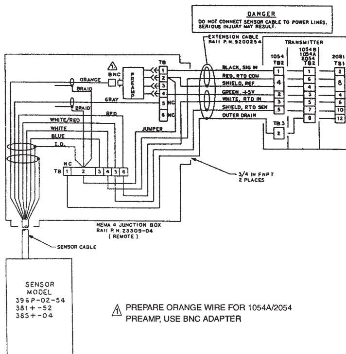
FIGURE 4-22. Wiring Details Model 396P-02-54 for use with Junction Box (PN 23309-04) and Remote Preamplifier (PN 22698-03), Extension Cable (9200254).
