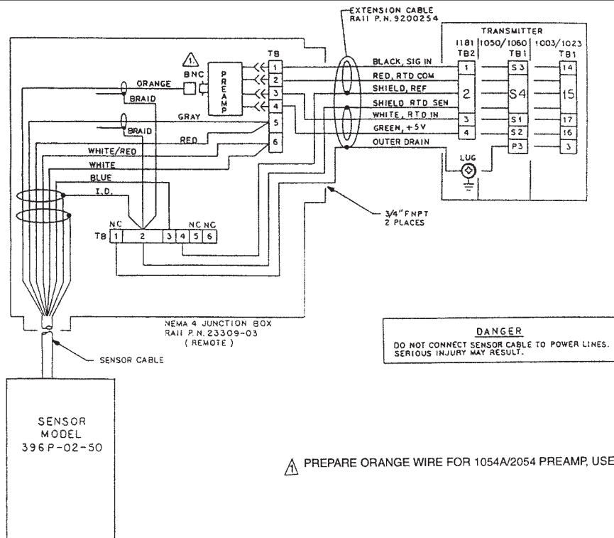
FIGURE 4-21. Wiring Details Model 396P-02-50 for use with Junction Box (PN 23309-03) and Remote Preamplifier, Extension Cable (PN 9200254).
