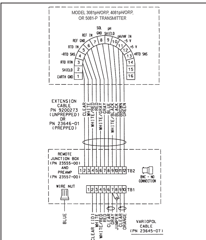
FIGURE 4-12. Wiring Details for Models 396PVP or 396P-02-55 with Mating Variopole Cable (PN 23645-07) for use with Remote Junction Box (PN 23555-00) to Models 3081, 4081, & 5081
