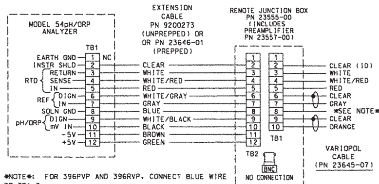
FIGURE 4-10. Wiring Details for Models 396PVP or 396P-02-55 with Mating Variopole Cable (PN 23645-07) for use with Remote Junction Box (PN 23555-00) to Model 54/54e
