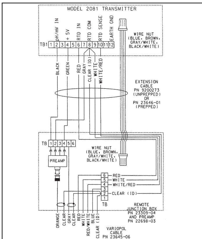
FIGURE 4-11. Wiring Details for Models 396PVP or 396P-02-54 with Mating Variopole Cable (PN 23645-06) for use with Remote Junction Box (PN 23309-04) to Model 2081
