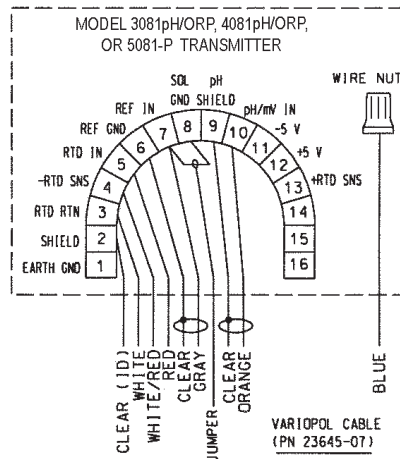
FIGURE 4-6. Wiring Details for Models 396PVP or 396P-02-55 with Mating Variopol Cable (PN 23645-07) for use with Models 3081, 4081, 5081
