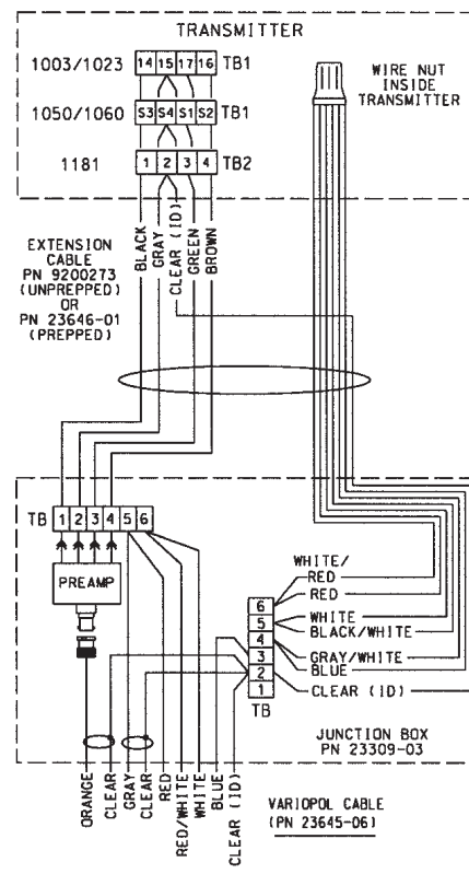
FIGURE 4-8. Wiring Details for Models 396PVP or 396P-02-50 with Mating Variopole Cable (PN 23645-06) for use with Remote Junction Box (PN 23309-03) to Model 1181
