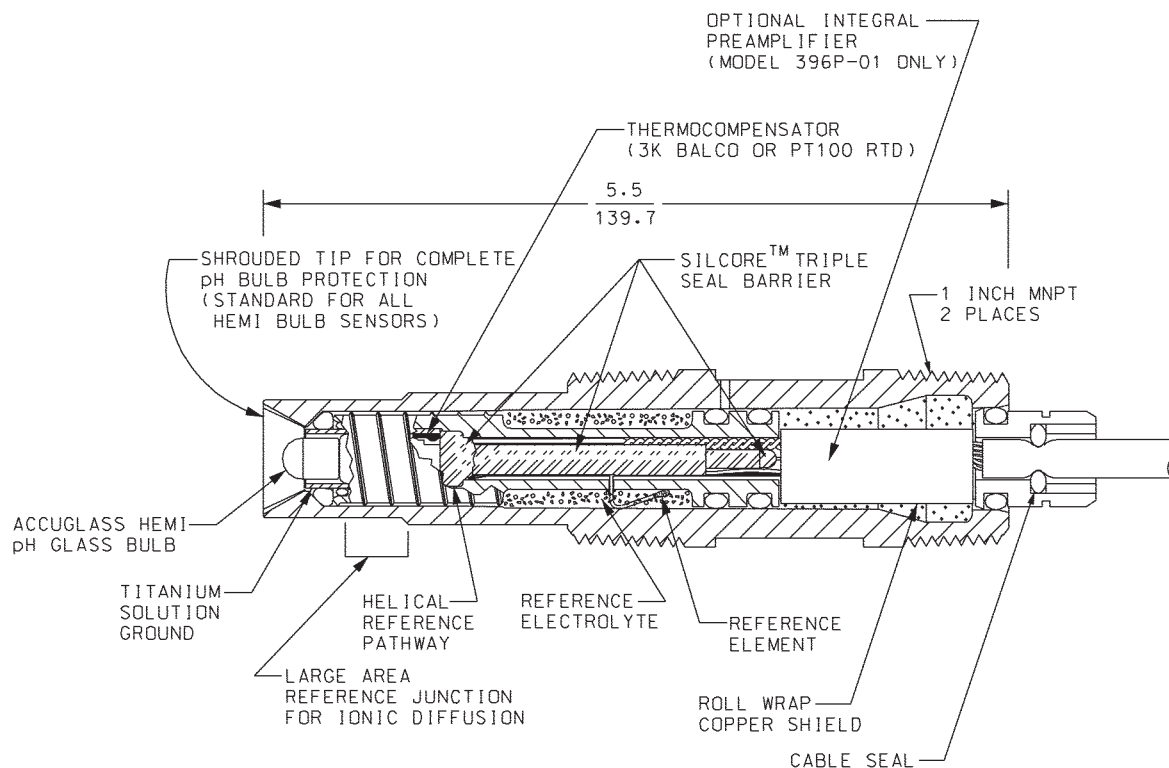
FIGURE 1-1. Cross Section Diagram of the TUpH Patented Reference Technology
