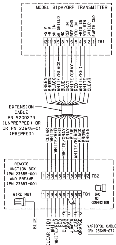
FIGURE 4-7. Wiring Details for Models 396PVP or 396P-02-55 with Mating Variopole Cable (PN 23645-07) for use with Remote Junction Box (PN 23555-00) to Model 81
