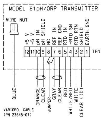
FIGURE 4-3. Wiring Details for Models 396PVP or 396P-02-55 with Mating Variopol Cable (PN 23645-07) for use with Model 81
