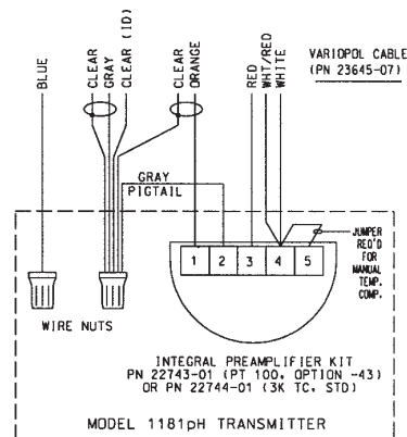
FIGURE 4-4. Wiring Details for Models 396PVP or 396P-02-50 with Mating Variopol Cable (PN 23645-07) for use with Model 1181
