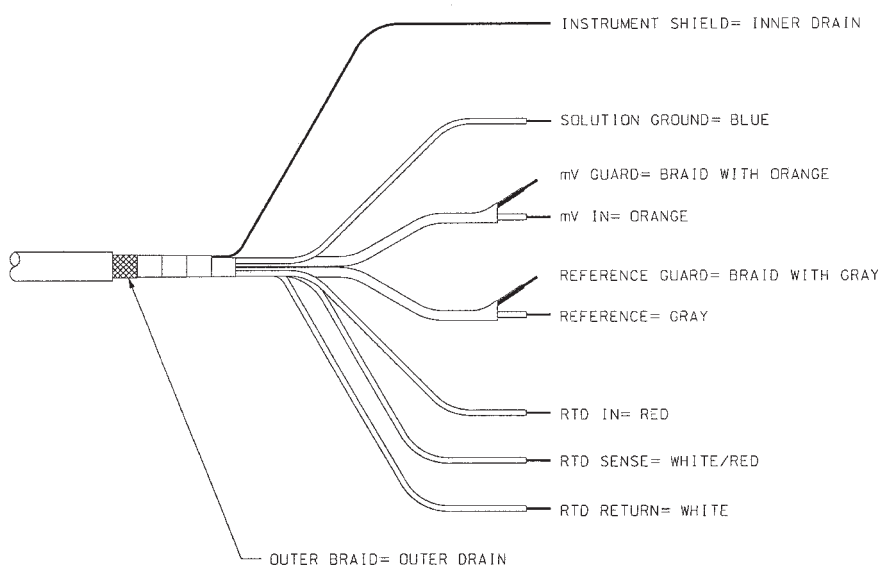
Model 396P Option 02 (without preamplifier) cable
