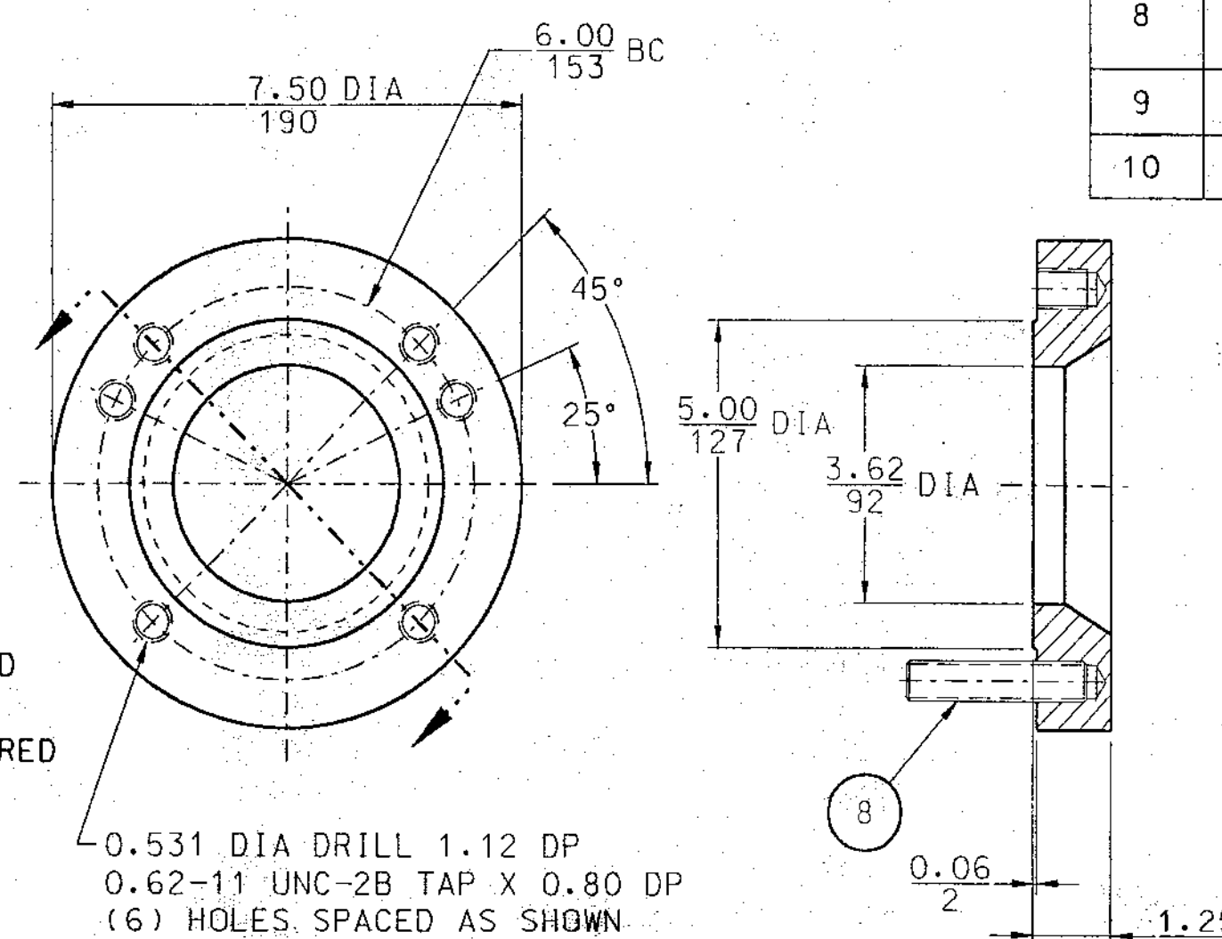
103 0 LEVEL TRANSMITTER FLANGE
