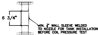
DETAIL A
