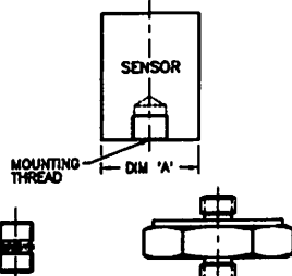
STANDARD MOUNTING STUD ELECTRICAL ISOLATION MOUNTING STUD/PAD (081A21 ONLY)
