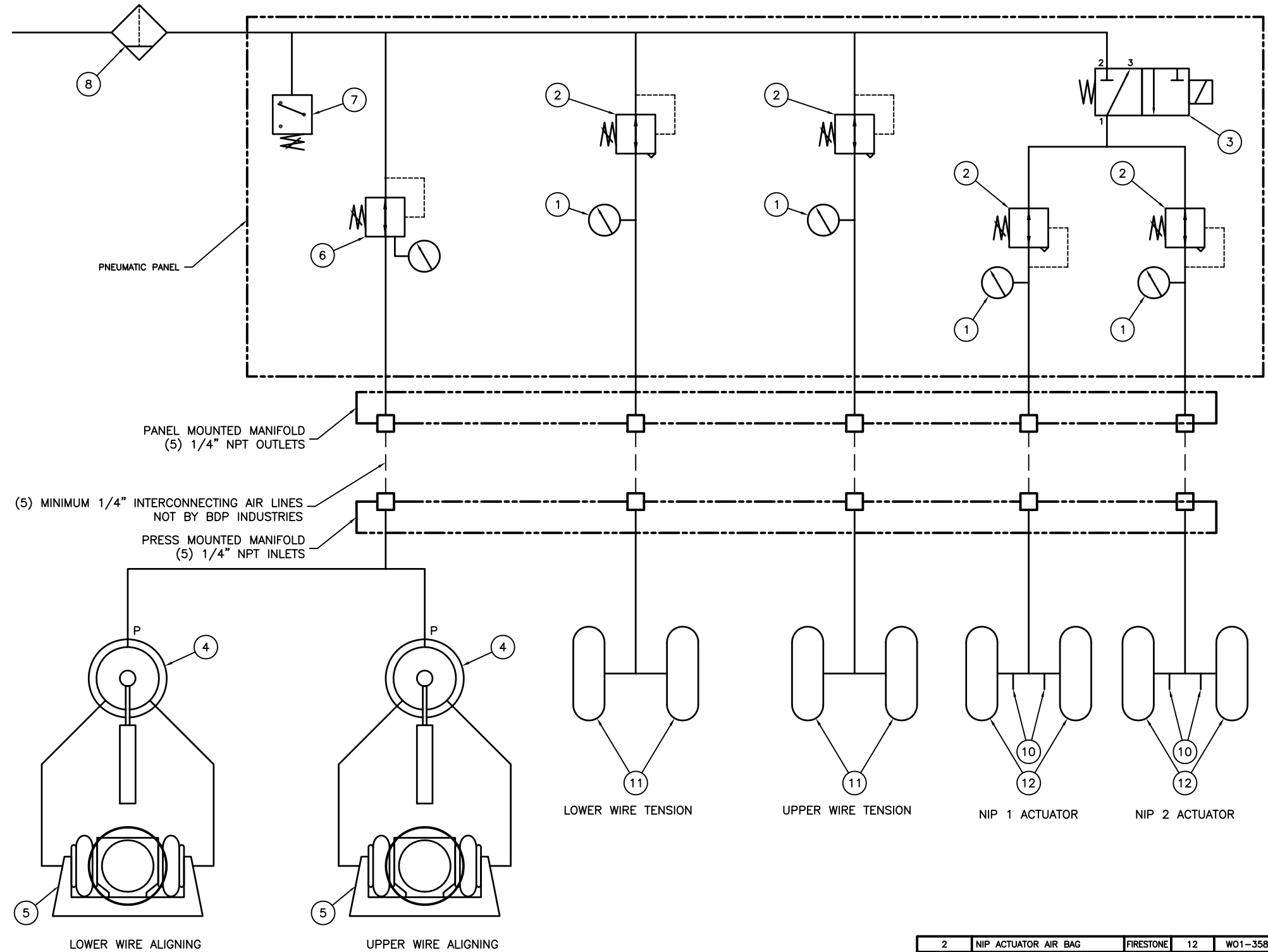
PNEUMATIC SCHEMATIC
