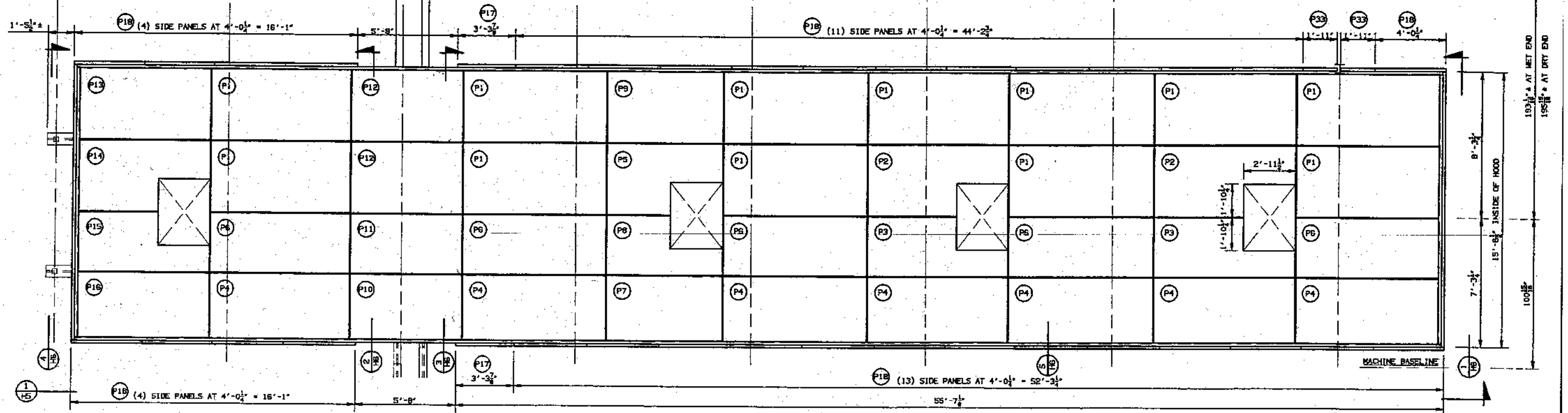
PLAN - NO. 1 P.M. DRYER SECTION HOOD PANELS
