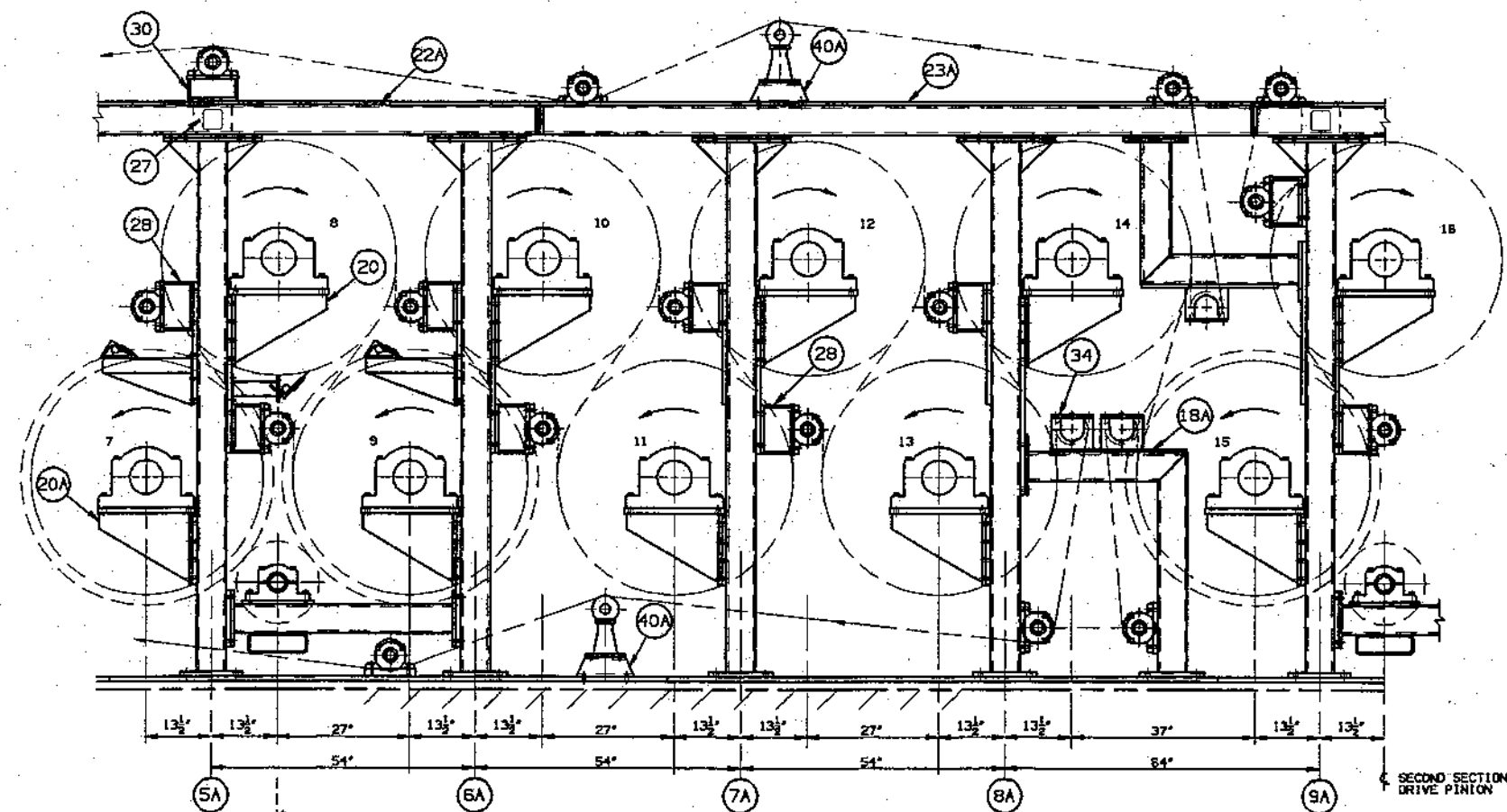
FIRST DRYER SECTION - D.S. DRYER FRAME ASSEMBLY
