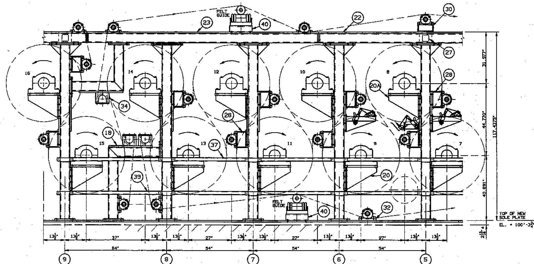
FIRST DRYER SECTION - T.S. DRYER FRAME ASSEMBLY
