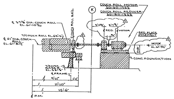
SECTION C-C SCALE 1/4"=1'-0" 50-13-1061
