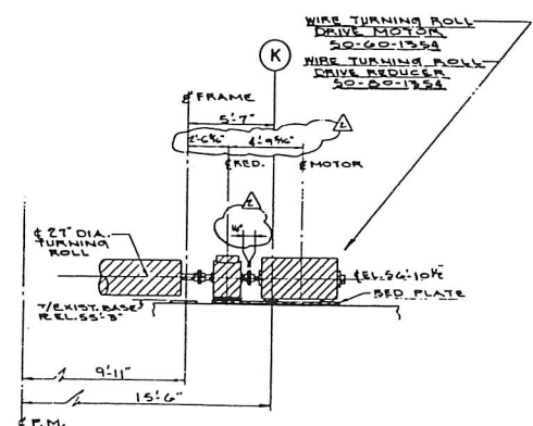
SECTION D-D SCALE 1/4"=1'-0" 50-13-1061
