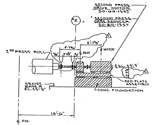
SECTION F-F SCALE 1/4"=1'-0" 50-13-1061
