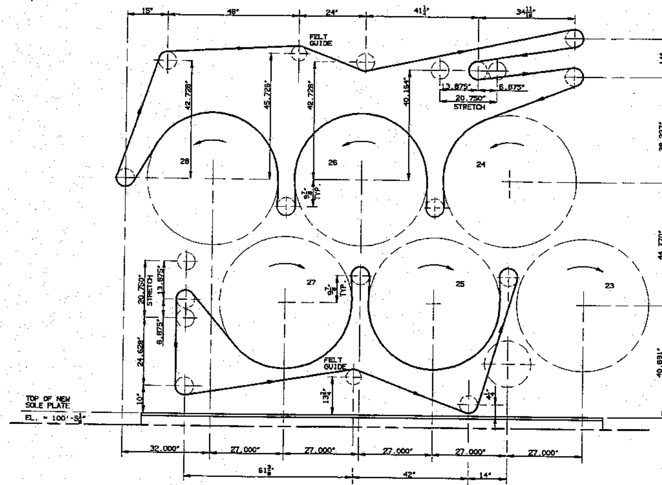
THIRD DRYER SECTION - PROPOSED FELT RUNS TOP FELT LENGTH 34'-0" BOTTOM FELT LENGTH 48'-6" 3/4" = 1'-0"
