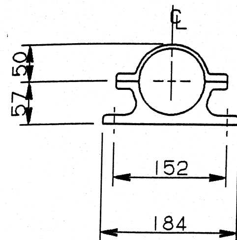
MOUNTING BASE DIMENSIONS
