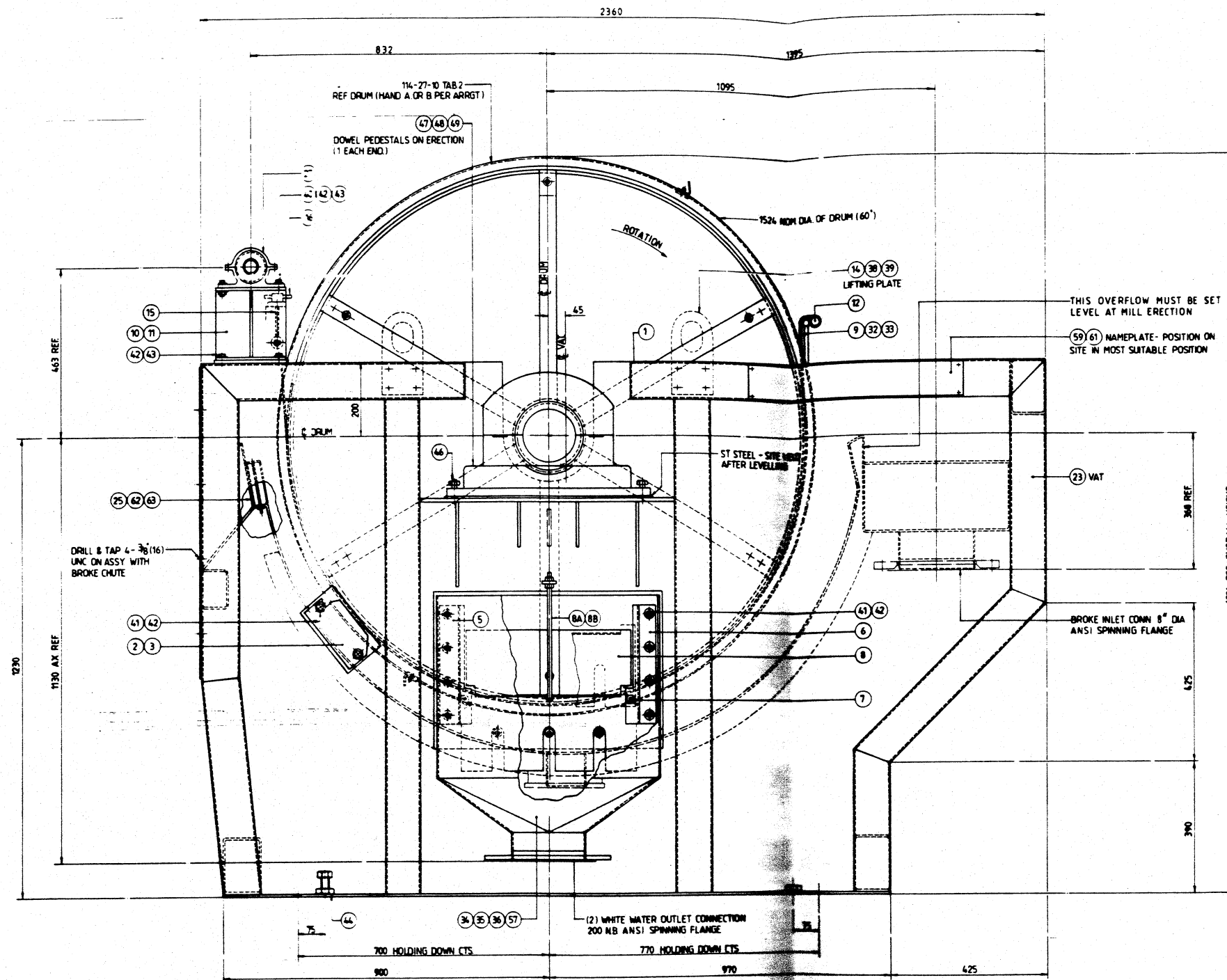
FRONT ELEVATION (SHOWING DRIVE ASSEMBLY 'A')
