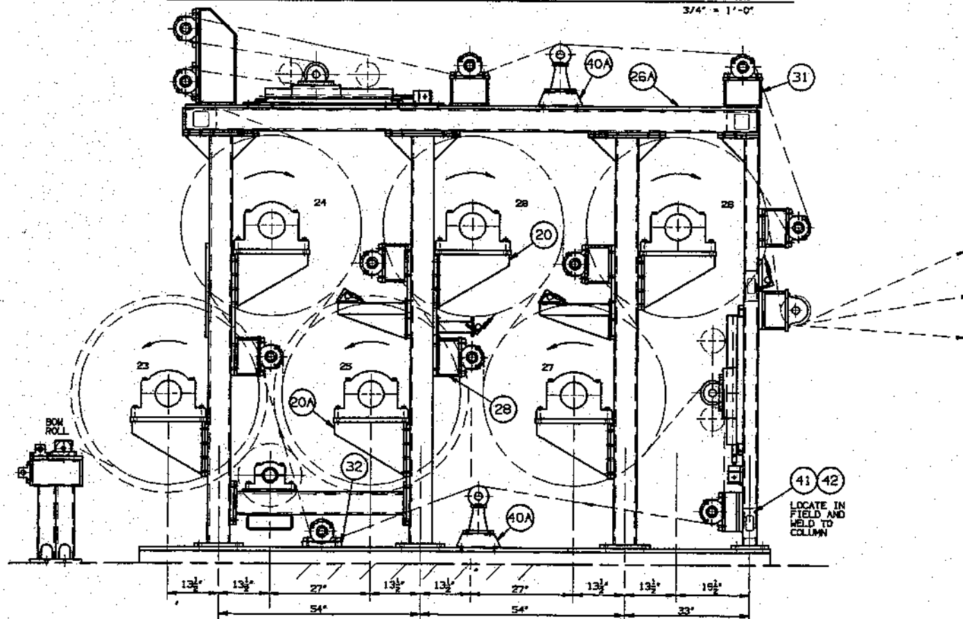
THIRD DRYER SECTION - D.S. DRYER FRAME ASSEMBLY
