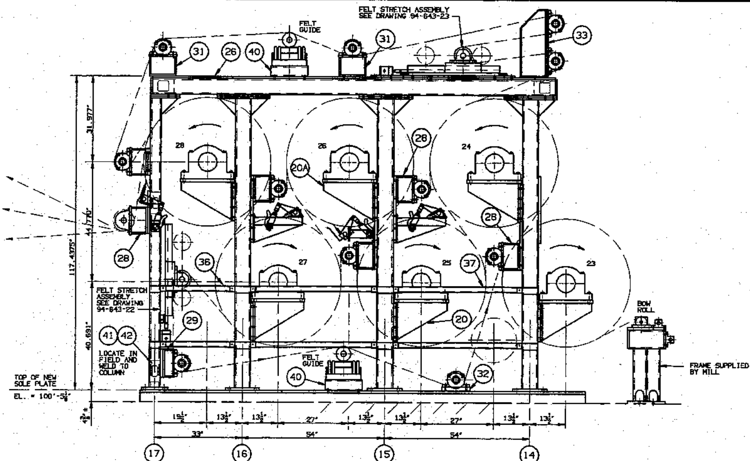
THIRD DRYER SECTION - T.S. DRYER FRAME ASSEMBLY
