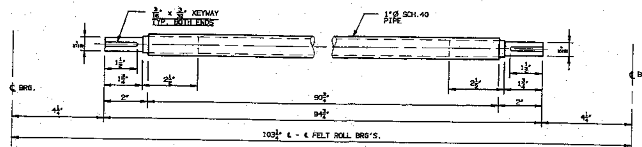
⑨ FELT STRETCH CROSS SHAFT DETAIL
