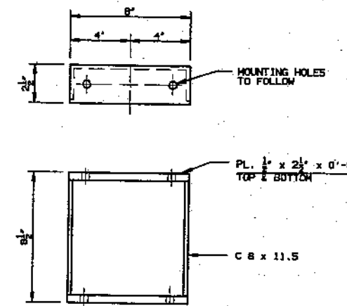
(44) SIZE PRESS PAPER ROLL BRACKET DETAIL
