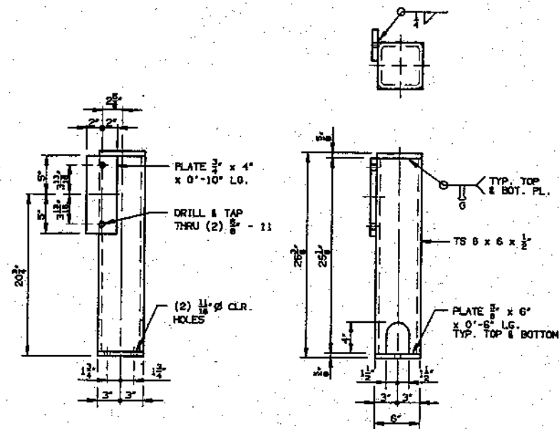
(35) MACHINE FRAME DETAIL
