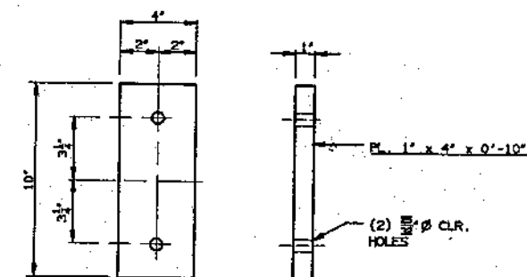
(45) FELT ROLL BRACKET SPACER PLATE DETAIL
