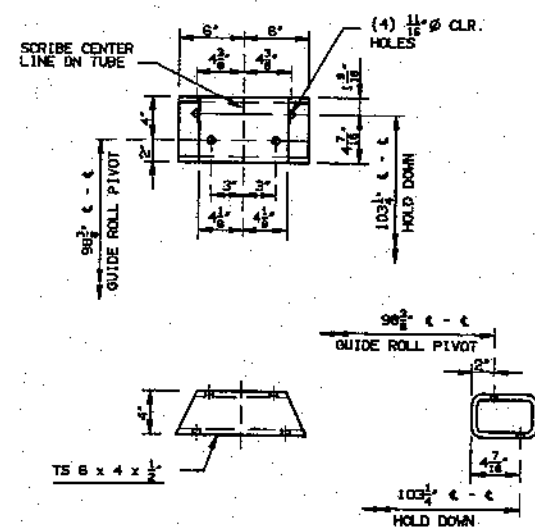
(40A) GUIDE ROLL BRACKET SUPPORT - DRIVE SIDE
