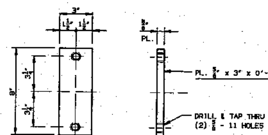
(42) SPACER PLATE DETAIL
