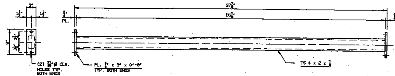
(41) MACHINE FRAME SPACER BAR DETAIL
