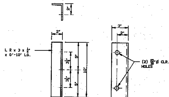
(43) SPRING ROLL BRACKET DETAIL
