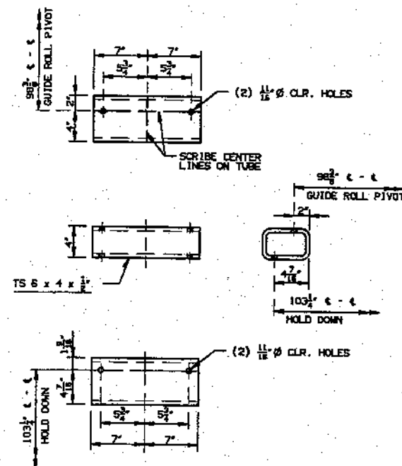
(40) GUIDE ROLL BRACKET SUPPORT - TENDING SIDE
