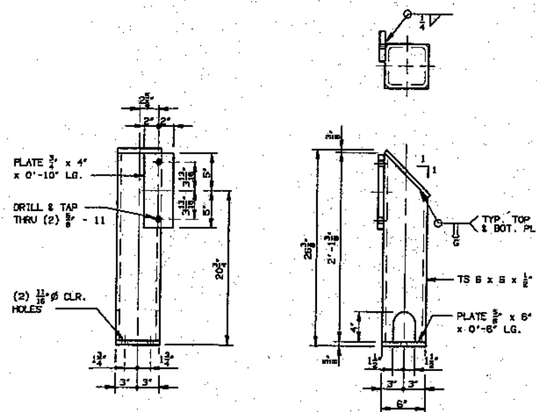
(35A) MACHINE FRAME DETAIL
