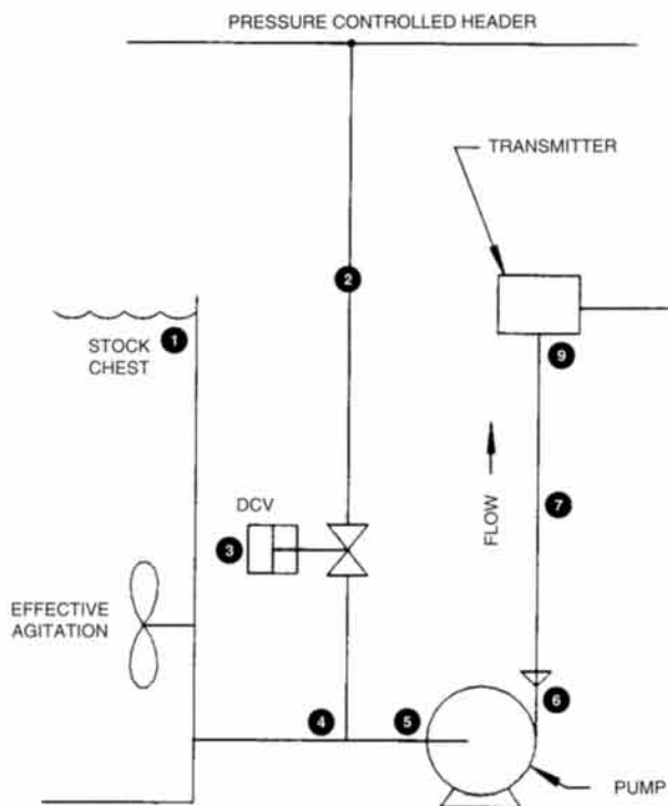
Vertical Installation
