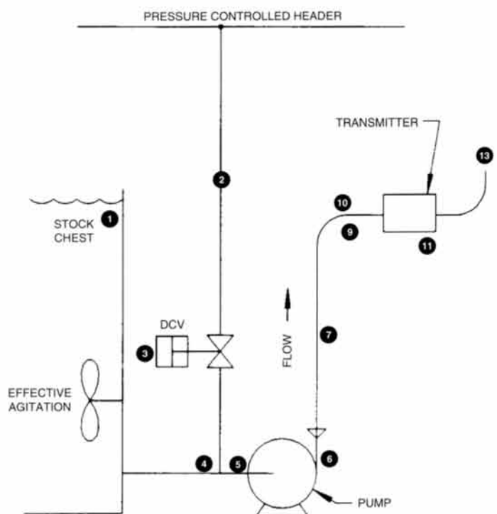
Horizontal Installation
