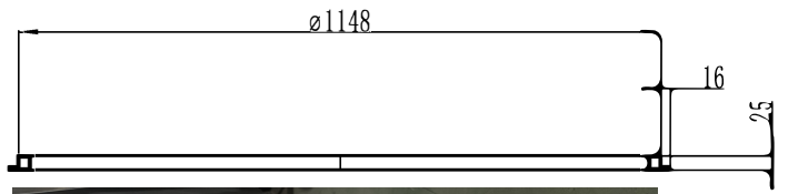
Screen Diameter
