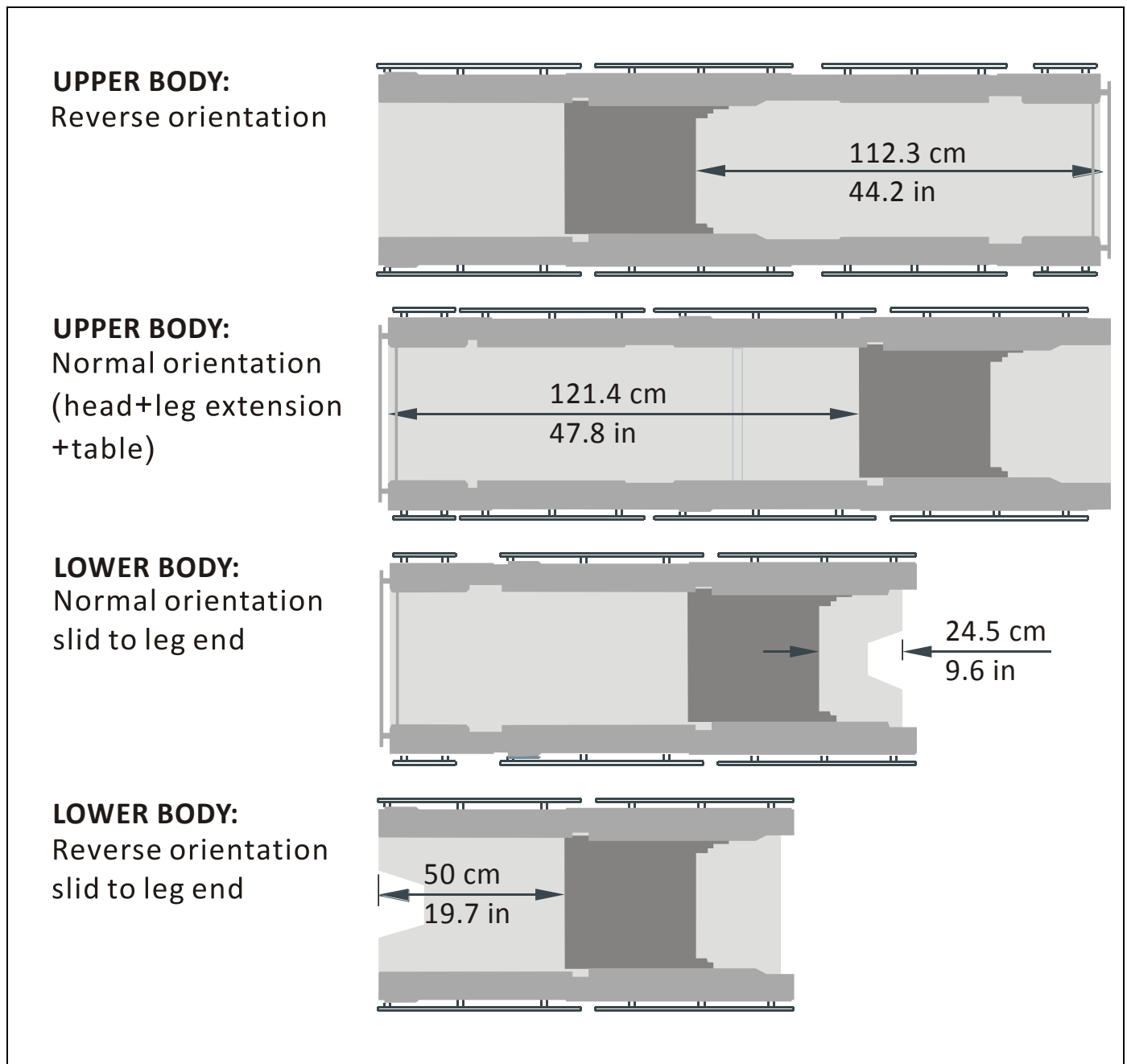
Figure 3-4-1: Models B2AV1000/B2AV1000K
