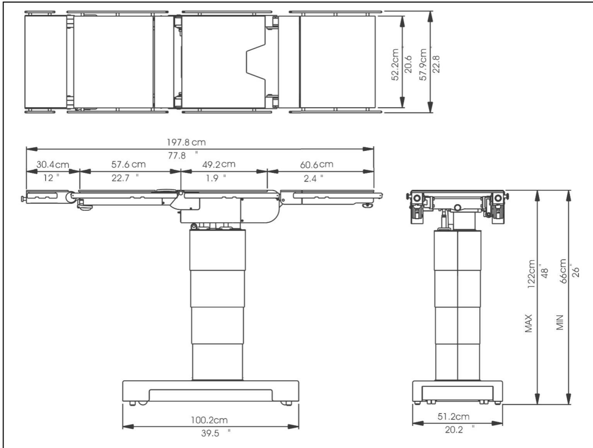
Figure 3-3: Dimensions
