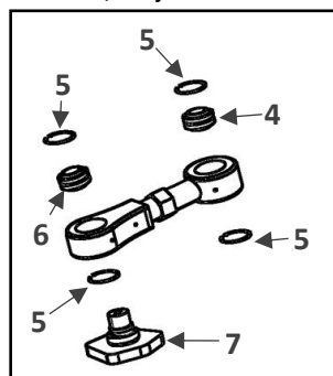
J Models w/ Adjustable Pitch Link
