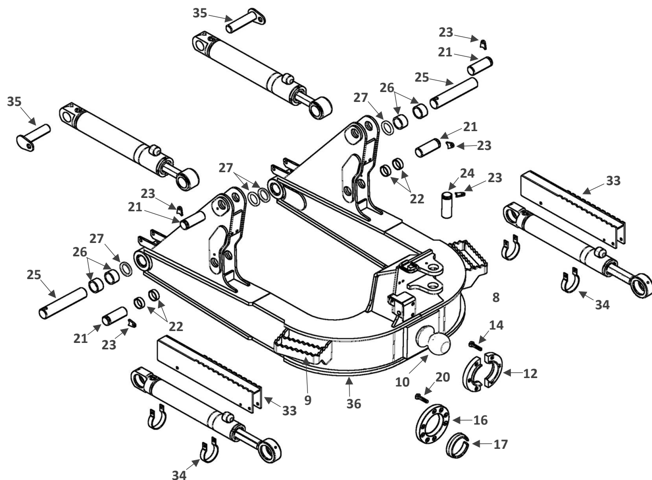
J Models w/ Adjustable Pitch Link
