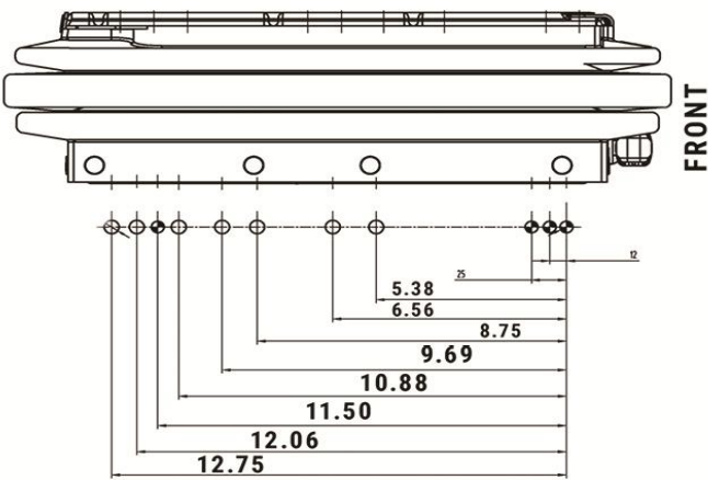
Variable Mounting Options
