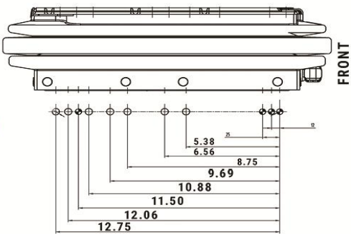
Variable Mounting Options
