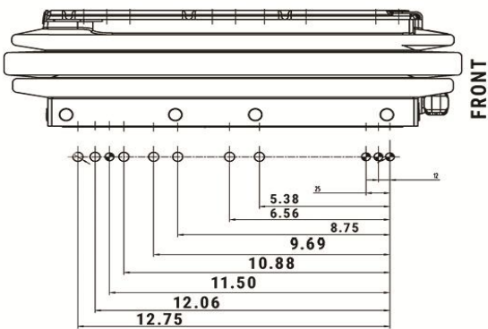
Variable Mounting Options
