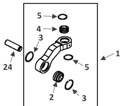
H Models w/ Fixed Pitch Link
