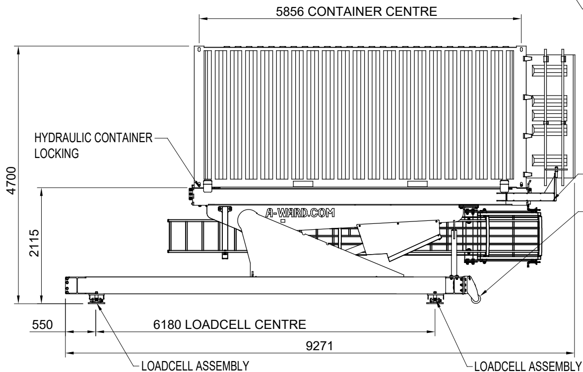
ELEVATION - HORIZONTAL
