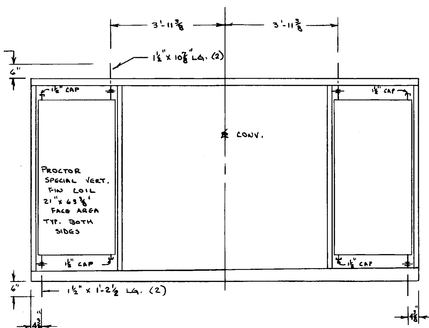
CROSS SECTION (VIEW FROM FEED END)
