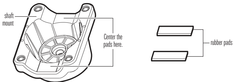
Shaft Mount Rubber Pad Placement
