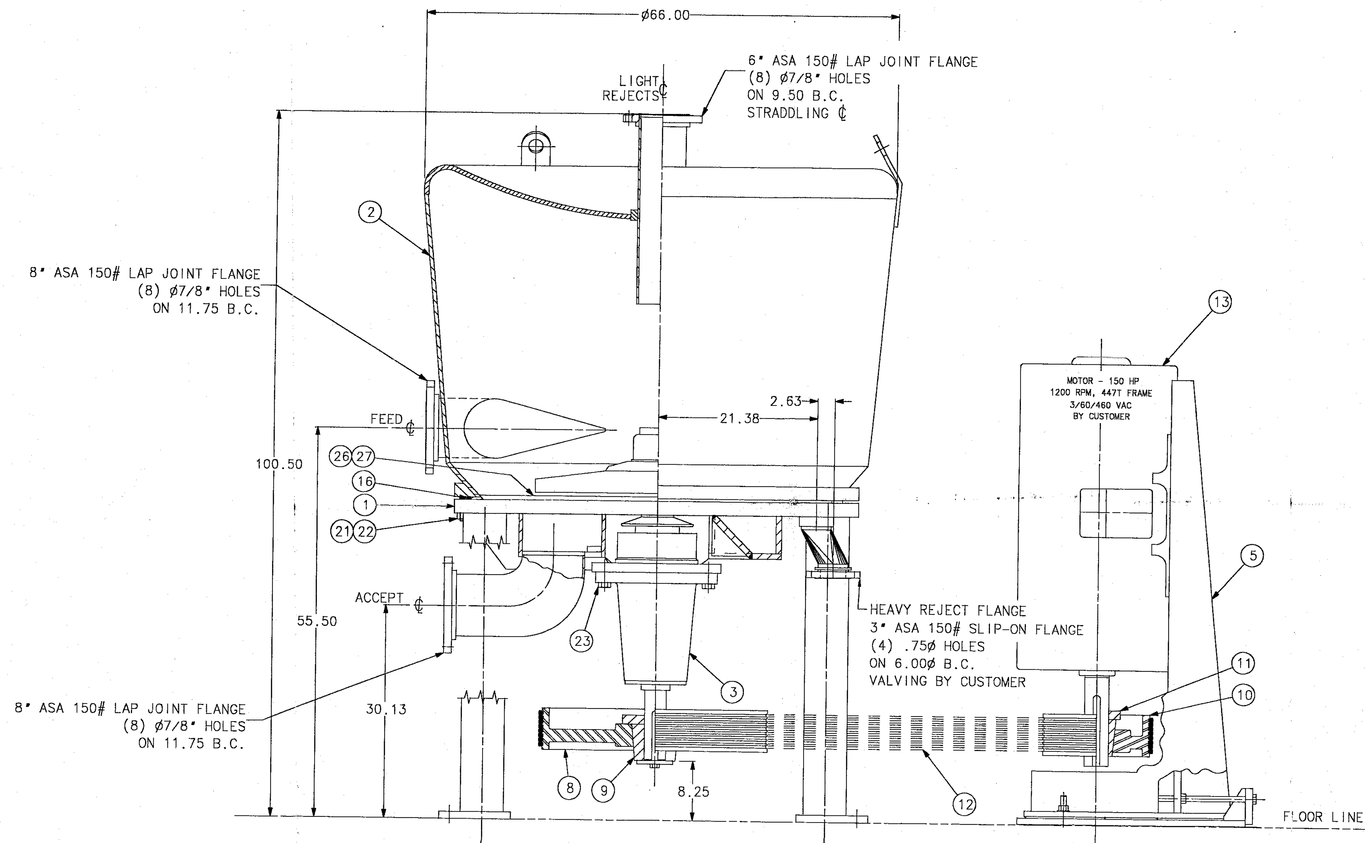
TYPICAL ELEVATION ALL PARTS NOT SHOWN IN TRUE VIEW REMOVED GUARDS FOR CLARITY
