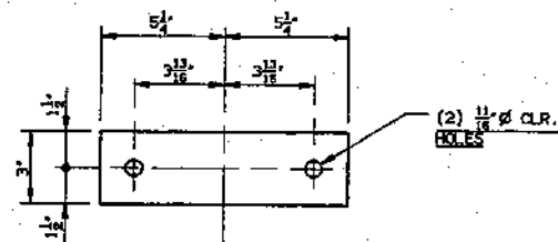
33 TOP FELT ROLL - SPACER BRACKET (6) REQ'D AS SHOWN MAT'L C.R.S.
