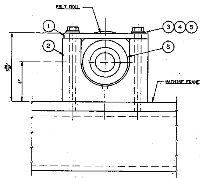
34 FELT ROLL BEARING HOUSING ASSEMBLY (8) ASSEMBLIES REQ'D 3/8 SCALE
