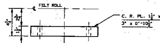
32 BOTTOM FELT ROLL - SPACER PLATE (8) REQ'D AS SHOWN
