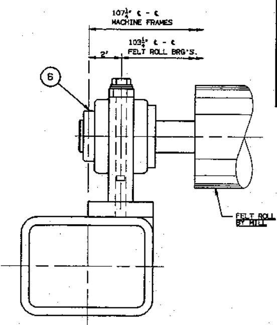
34 FELT ROLL BEARING HOUSING ASSEMBLY (8) ASSEMBLIES REQ'D 3/8 SCALE
