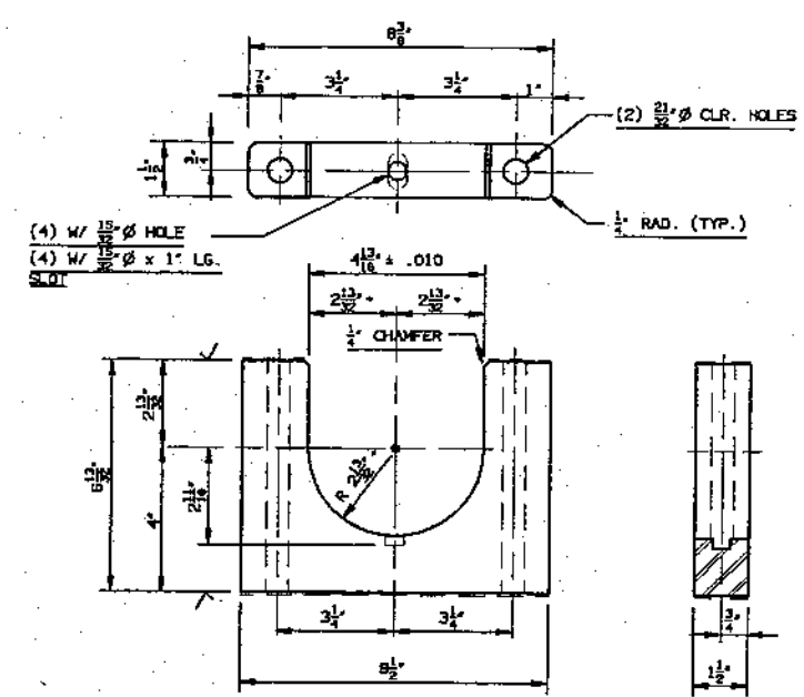
2 BEARING HOUSING DETAIL (8) REQ'D.
