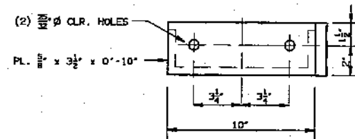
33 TOP FELT ROLL - SPACER BRACKET (6) REQ'D AS SHOWN MAT'L C.R.S.
