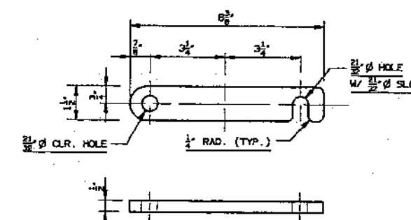
1 BRG. HOLD-DOWN CAP DETAIL (6) REQ'D.
