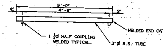
TENDING SIDE - 3" S.S. HEADER
