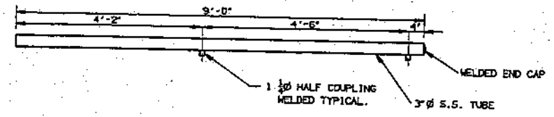
DRIVE SIDE - 3" S.S. HEADER
