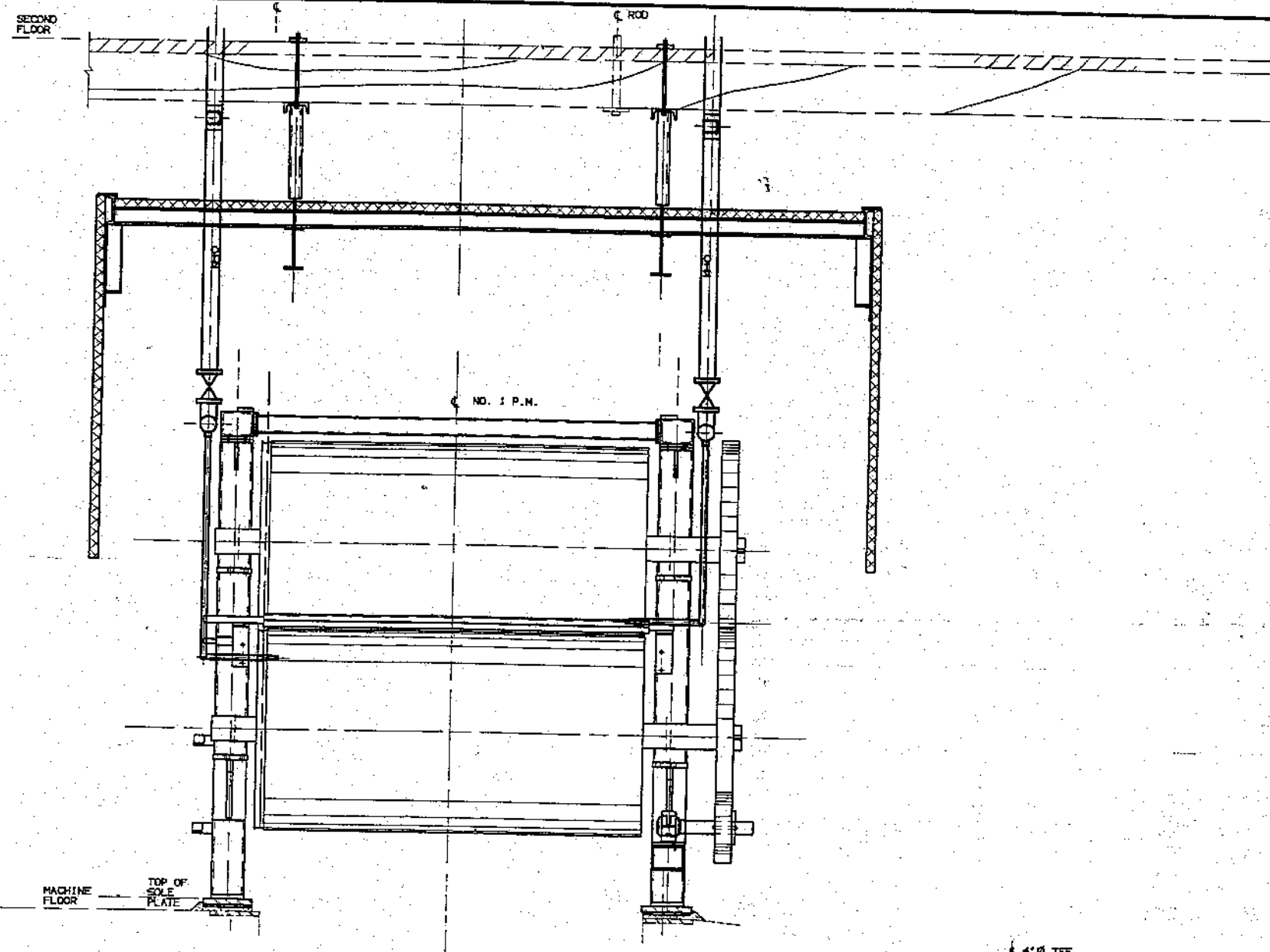
POCKET VENTILATION - MACHINE CROSS SECTION
